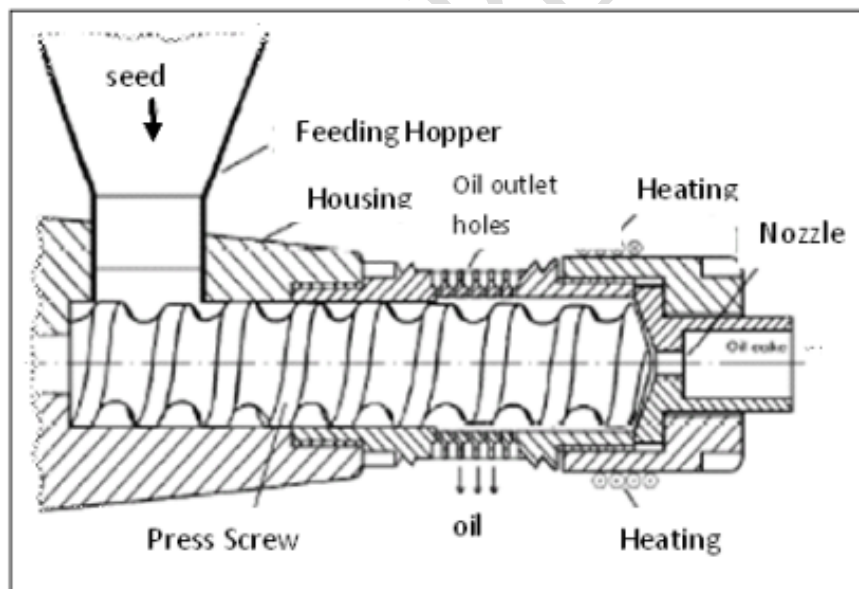
Fig. 3. Hole cylinder press of a KOMET oil expeller [19]
