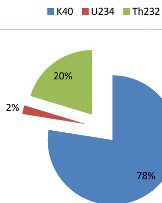
Figure 1: Percentage Contribution of Radionuclide in Transfer Factor
