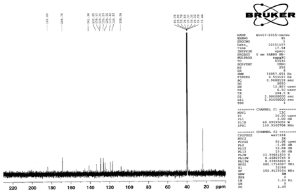
Figure 5. 13 Cnmr spectrum of the Chelator-ligand
