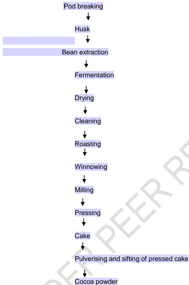
Figure 1: Flow chart for cocoa powder
