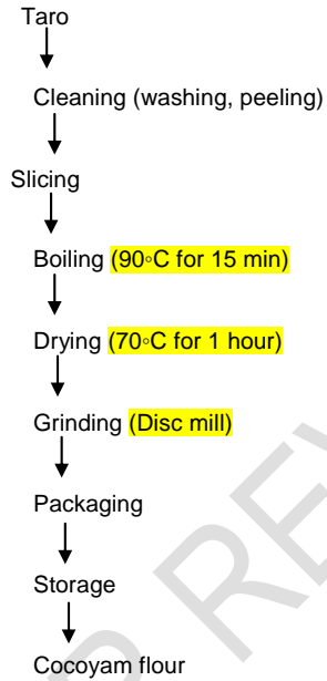
Fig.1: Flow diagram of cocoyam flour production modified from Mbanali et al. (2019)
