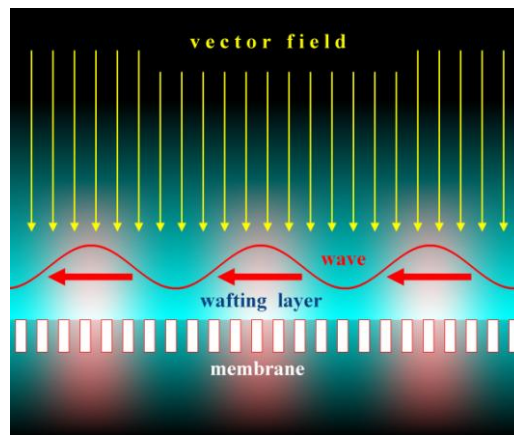
Fig. 1: Membrane with wafting layer, wave and vector field
