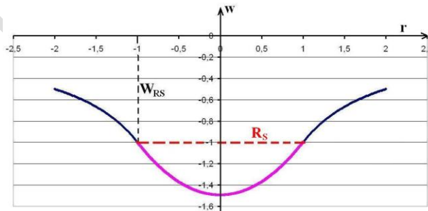
Fig. 4: Shape of the gravitational funnel
