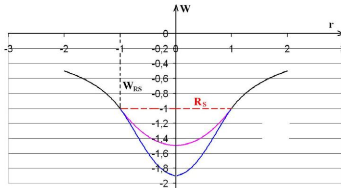
Fig. 5: Shapes of the depth of space
