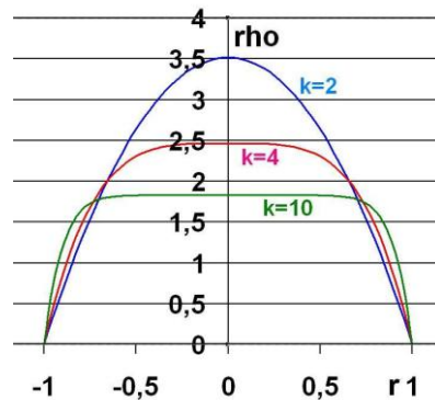
Fig. 7: Courses of density \rho in 1000 \text{ kg/m}^3 for various values of k
