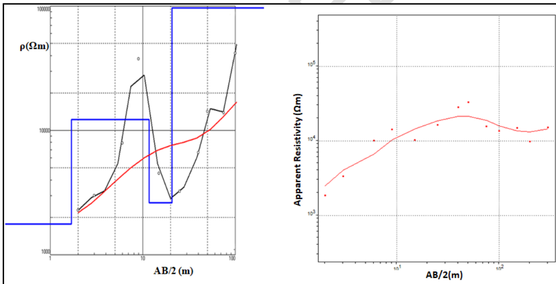
Figure 2a: Typical Sounding curves at VES point 1 of the study area.
