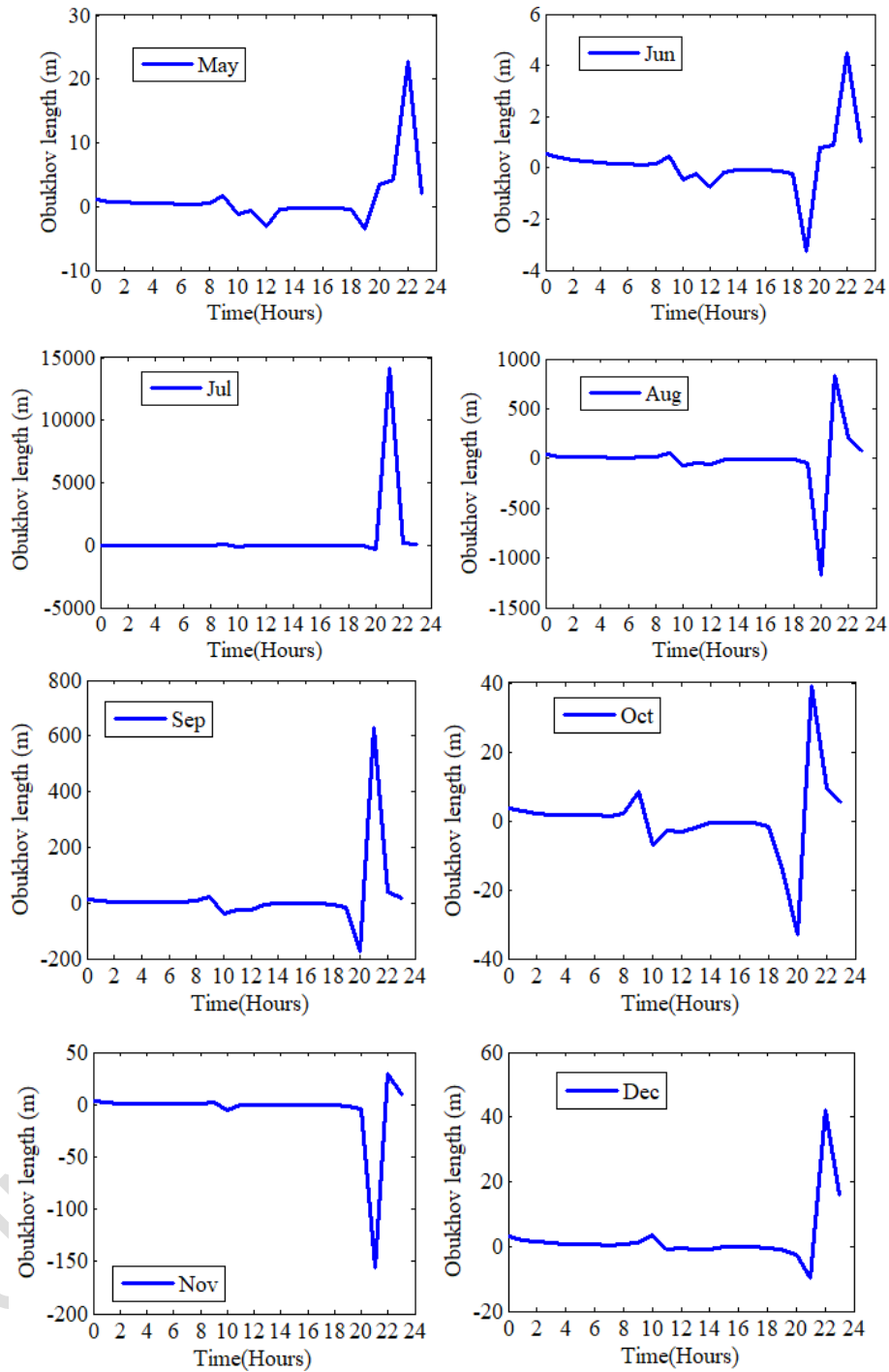
Fig. 6. Monthly variation of Obukhov length in Conakry (2001-2019)
