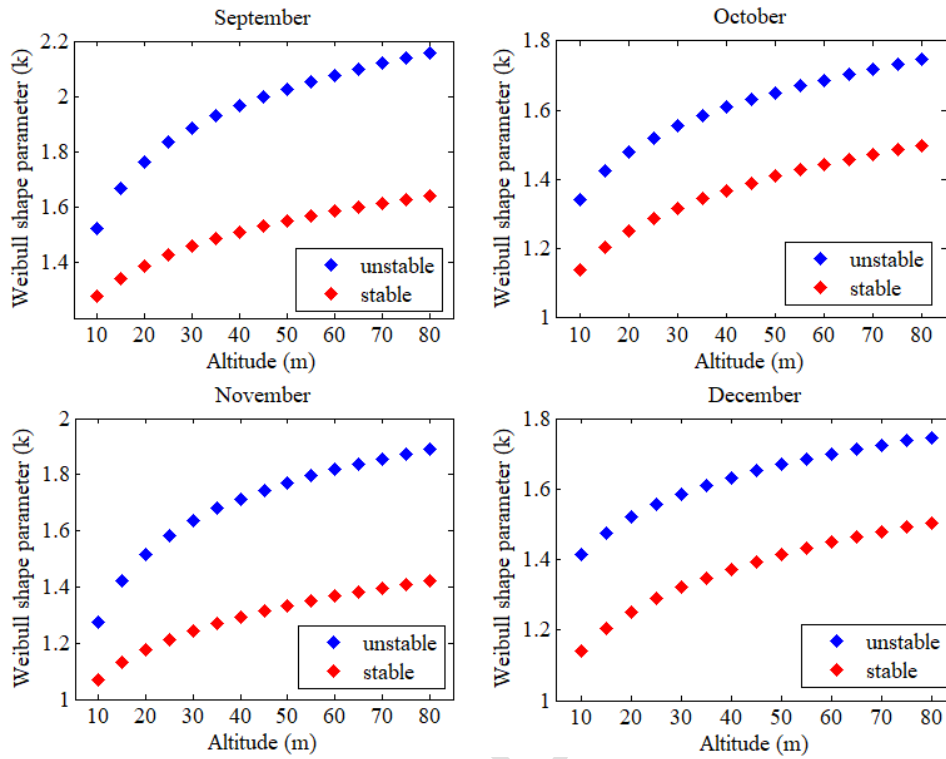
Fig. 11. Monthly variation of k during the stable and unstable period of the atmosphere in Conakry (2001-2019)
