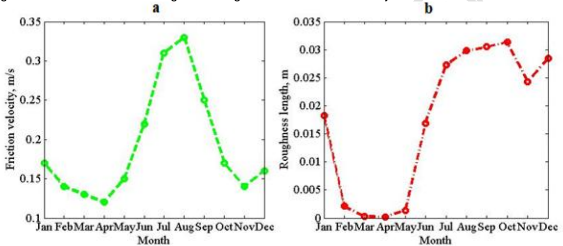
Fig. 5. Monthly variation of ground roughness and friction velocity in Conakry (2001-2019)
