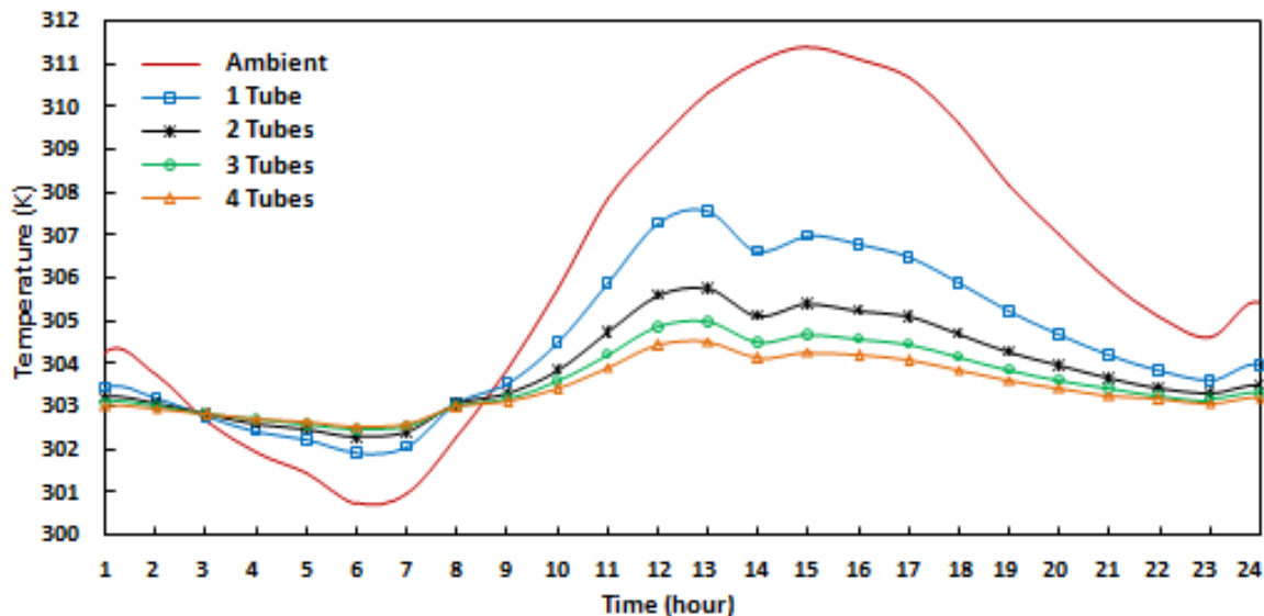
Figure 6: Effect of number of tubes on air temperature in habitat during April
