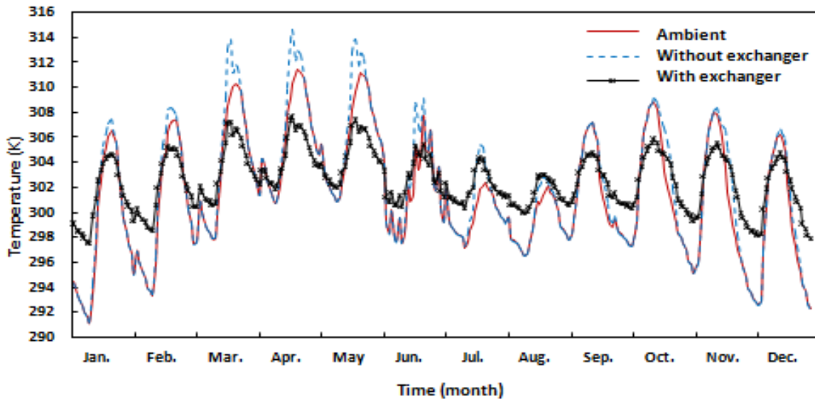
Figure 3: Effect of Canadian well on air temperature in habitat during a year
