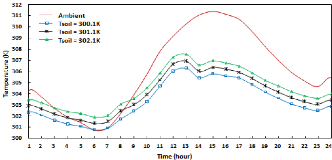
Figure 5: Effect of soil temperature on air temperature in habitat during April
