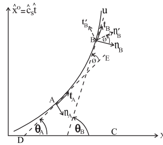
Figure 2: A one-dimensional metric space curving onto the absolute time ‘dimension’ along the vertical, projects a straight line one-dimensional metric space along the horizontal.
