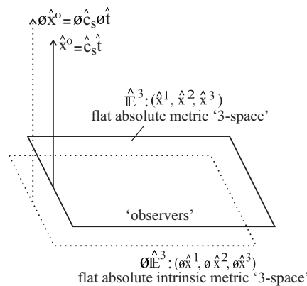
Figure 7: Flat ‘3-dimensional’ absolute metric space - absolute metric time is underlay by flat ‘3-dimensional’ absolute intrinsic metric space - absolute intrinsic metric time.
