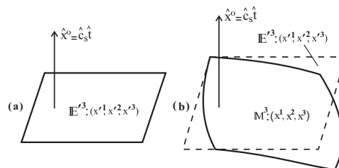
Figure 1: (a) Graphical representation of the Galileo space and (b) the Euclidean 3-space \mathbb{E}^3 of the Galileo space evolves into a curved 3-dimensional (Riemannian) metric space \mathbb{M}^3 , such that none of the dimensions of \mathbb{M}^3 spans the absolute time ‘dimension’ along the vertical.
