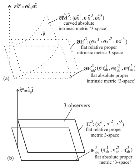
Figure 6: Figure 5 made more complete by including absolute proper metric ‘3-space’ \mathbb{E}_{ab}^3 as outward manifestation of \emptyset \mathbb{E}_{ab}^3 in Fig. 5 and the relative proper intrinsic metric 3-space \emptyset \mathbb{E}^3 that underlies \mathbb{E}^3 in Fig. 5.
