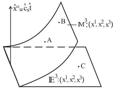
Figure 3: A 3-dimensional Riemannian metric space curving onto the absolute time ‘dimension’ along the vertical (as a curved hyper-surface) and its underlying projective Euclidean 3-space (as a flat hyper-surface) along the horizontal.
