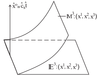
Figure 1: (c) The proper Euclidean 3-space \mathbb{E}^3 of the Galileo space evolves into a curved 3-dimensional (Riemannian) metric space \mathbb{M}^3 , such that the dimensions of \mathbb{M}^3 span the absolute time ‘dimensions’ \hat{c}_s \hat{t} along the vertical solely. The curved space \mathbb{M}^3 (as a curved hyper-surface), projects a new Euclidean 3-space \mathbb{E}^3 , with dimensions, x^1, x^2 and x^3 , underneath itself as a flat hyper-surface along the horizontal.
