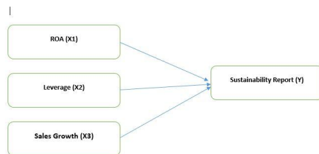
Fig 1: Framework
