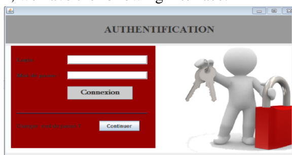
Fig 5: Authentication interface
