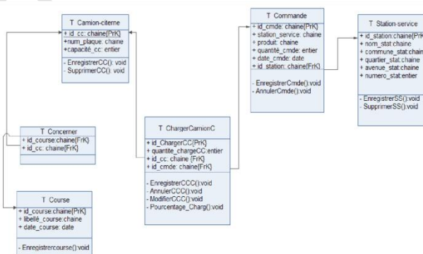
Fig. 4: Pseudo Logical Data Model
