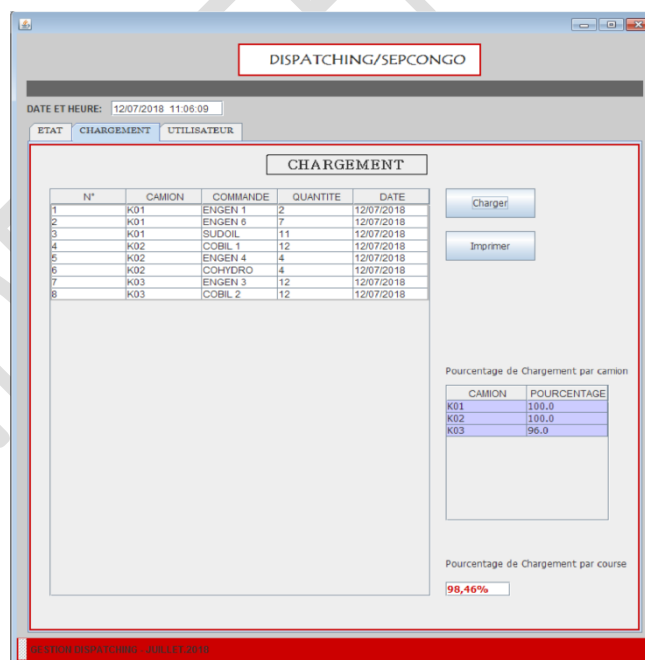
Fig 7: Loading results.
