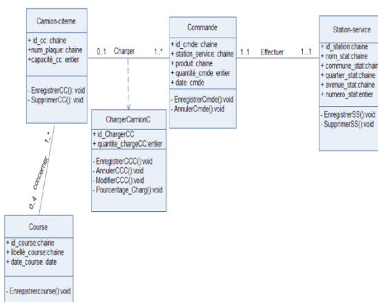
Fig 3: Class diagram
