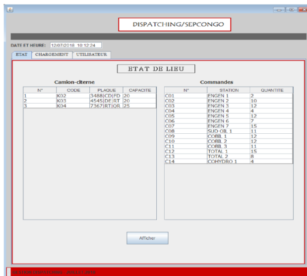
Fig 6: Main window.
