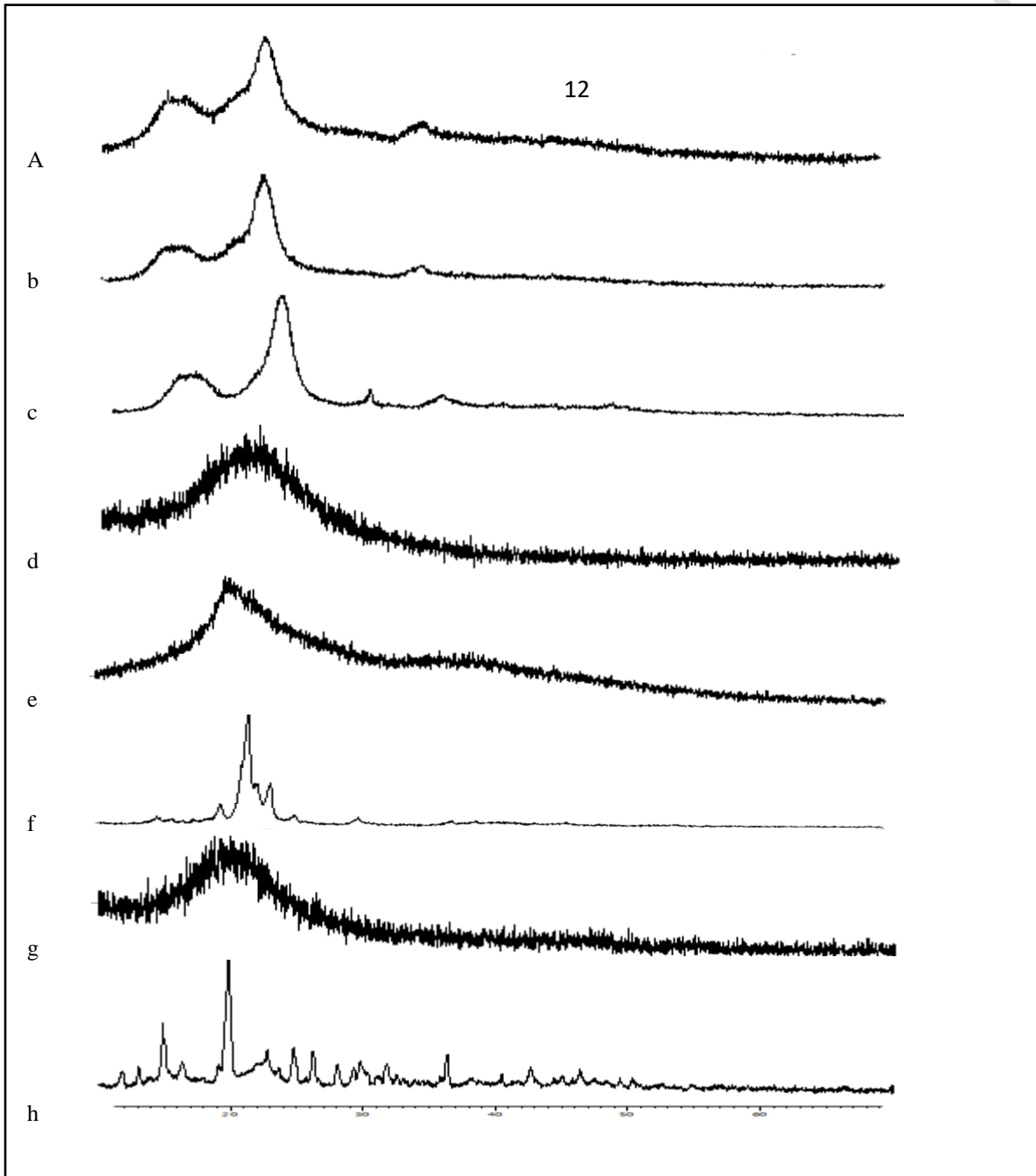
Fig. 3. XRD scanning of (a) liquisolid tablets (b) physical mixture F4 (c) Avicel (d) Aerosol (e) SCC (f)mg stearate (g) tween 20 [80%] (h) Pure haloperidol
