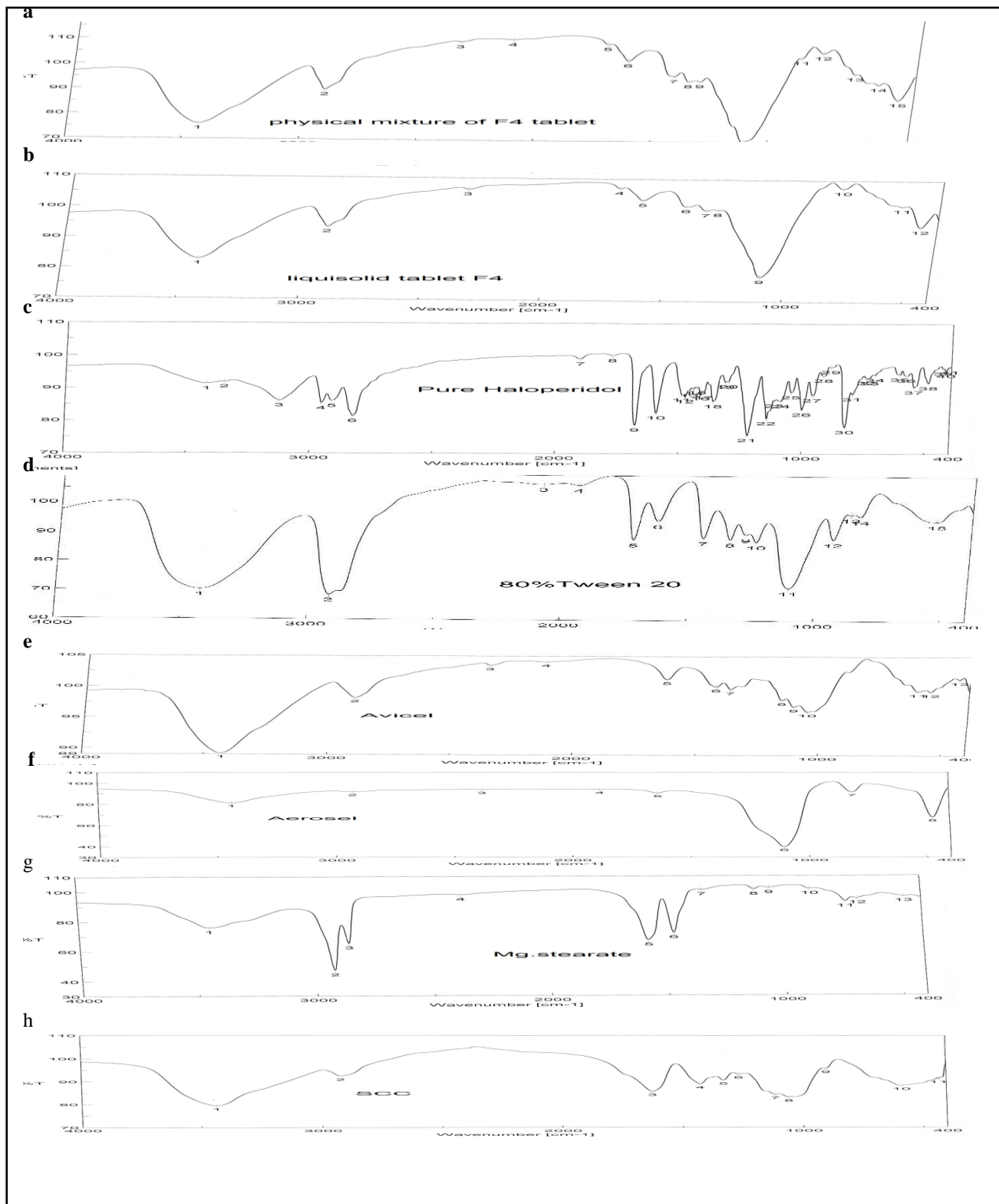
Fig. 1. IR spectra of (a) physical mixture of liquisolid formula (b) liquisolid formula F4 tablet (c) Pure haloperidol (d) tween 20 [80%] (e) Avicel (f) Aerosel (g) Mg.stearate (h) SCC
