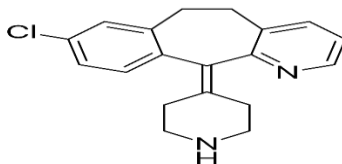
Figure 1. Chemical structures of DSL.
