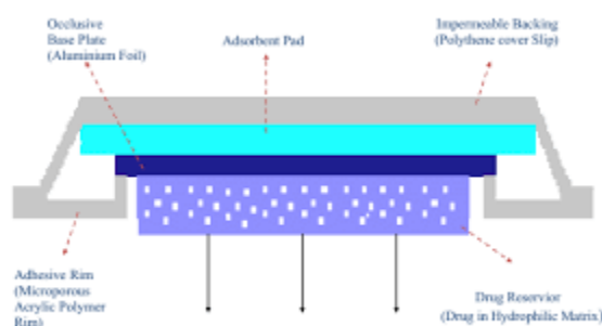
Figure .4 Micro reservoir transdermal patches
