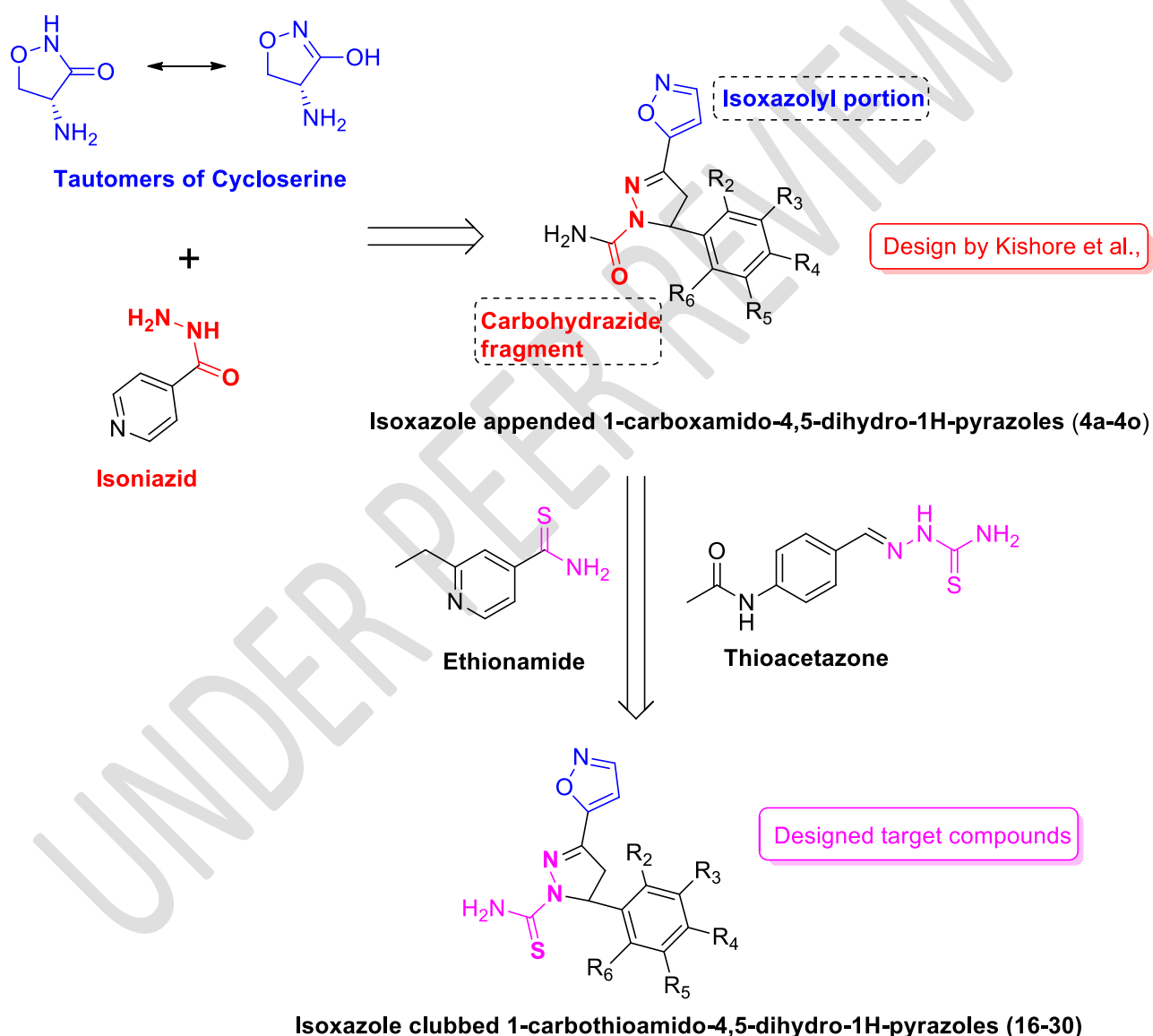
Figure 1. Design of isoxazole clubbed 1-carbothioamido-4,5-dihydro-1H-pyrazoles.
