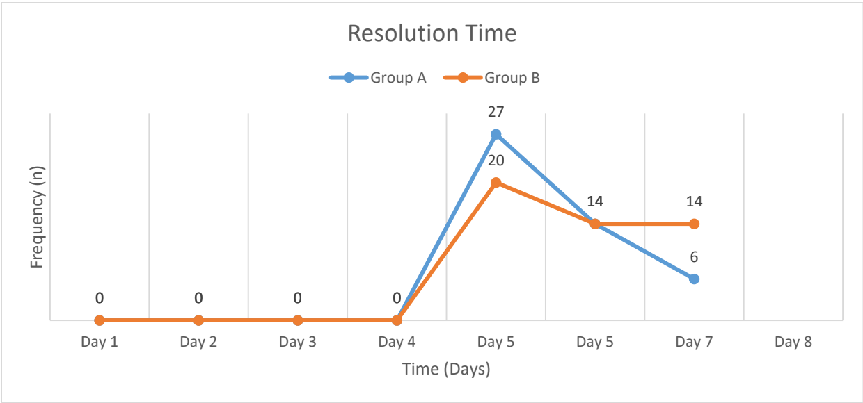
Fig 1 : Resolution Time
