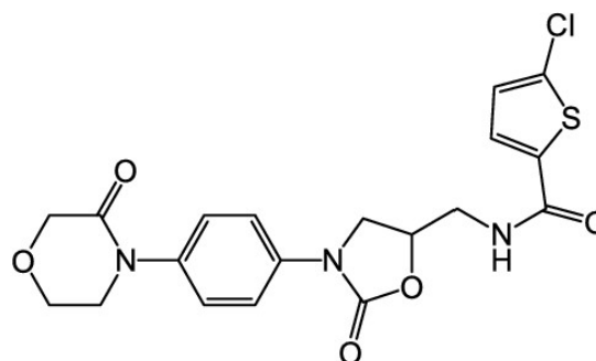
Figure 1: Structure of Rivaroxaban (3)
