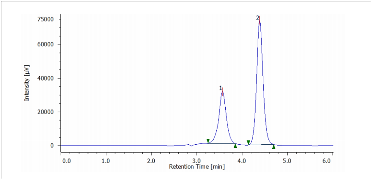
Fig 2. Chromatogram of standard solution
