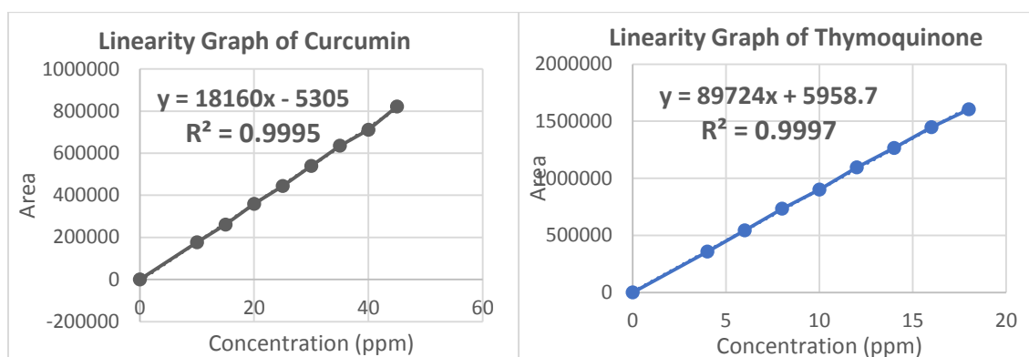
Fig4. Linearity graph of Curcumin and Thymoquinone
