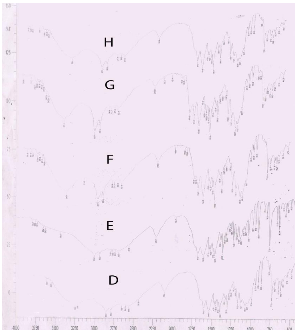
Figure:2 FT-IR Spectroscopy of formulation F1- F5.(D- F1, E- F2, F- F3, G-F4 and H -F5
