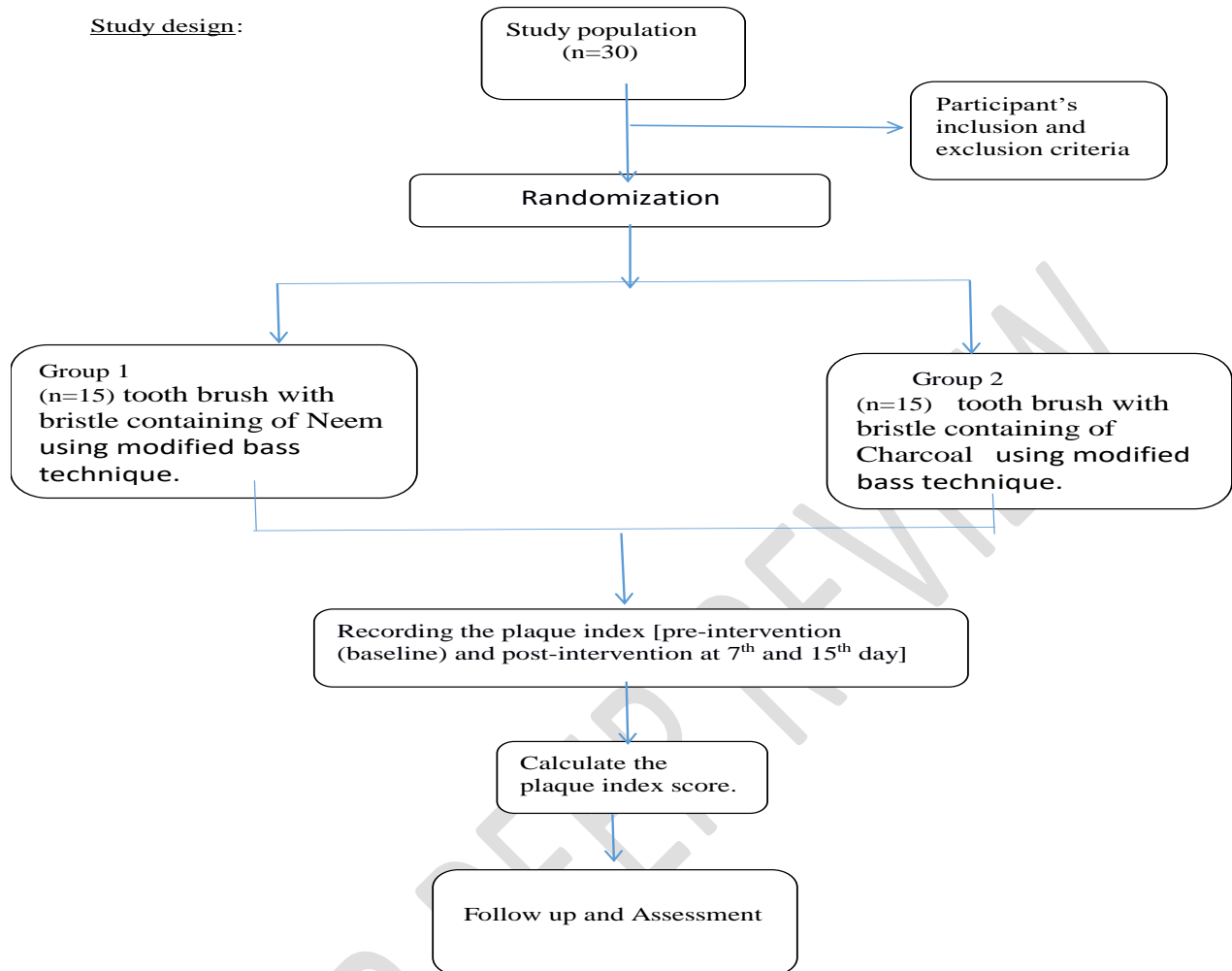
Fig. 1. Study design
