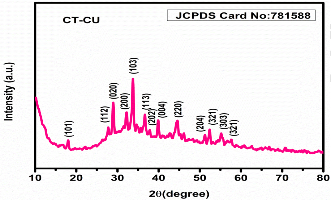
Figure 6: XRD pattern of green synthesized NPs from tuber extract of C. tuberosa
