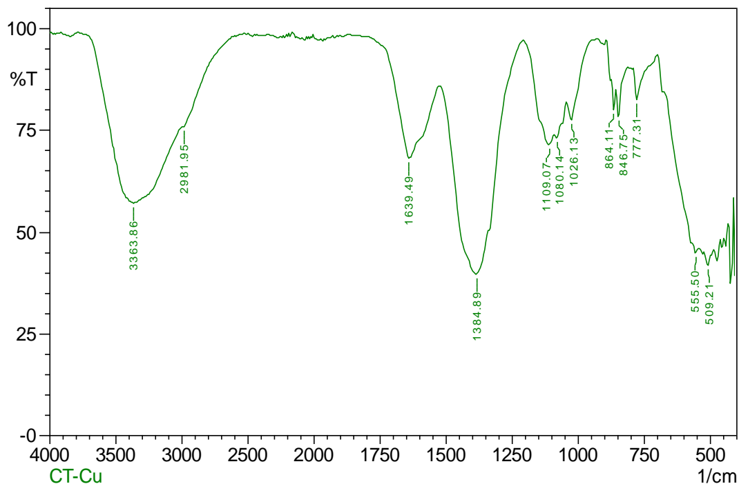
Figure 3: FTIR spectra of green synthesized CuONPs from tuber extract of C. tuberosa .
