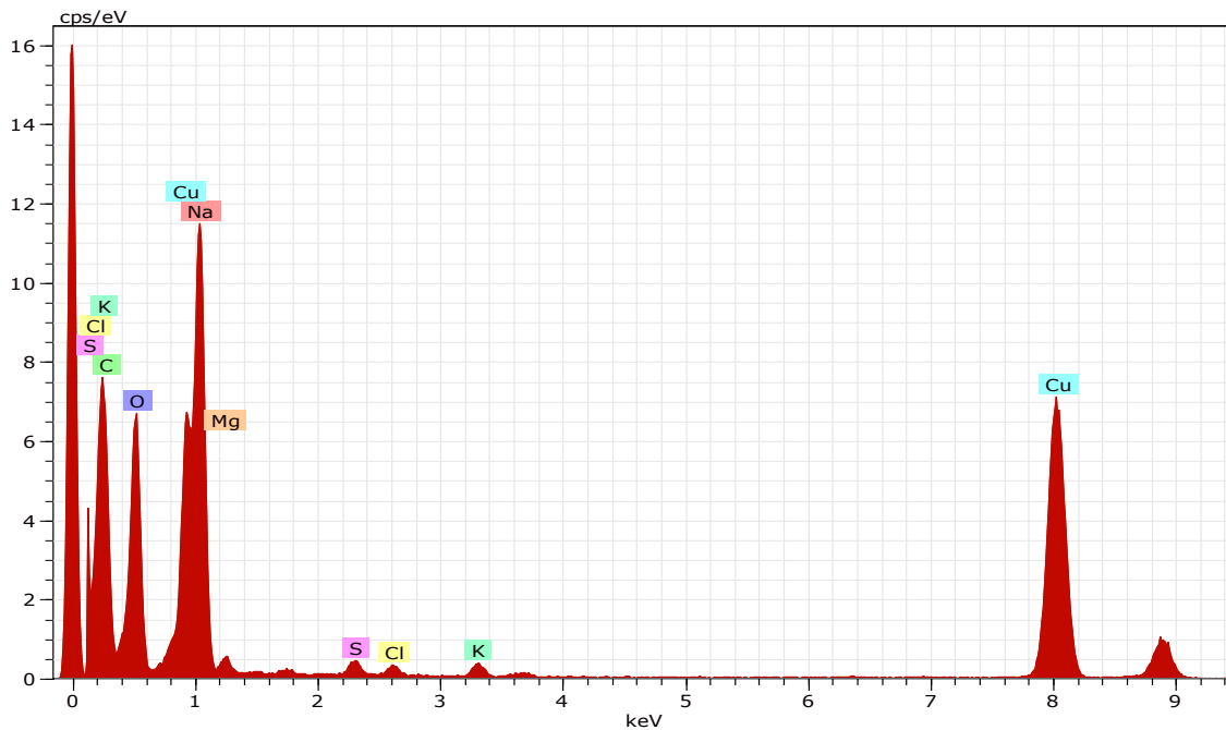
Figure 8: EDX spectrum of green synthesized NPs from tuber extract of C. tuberosa
