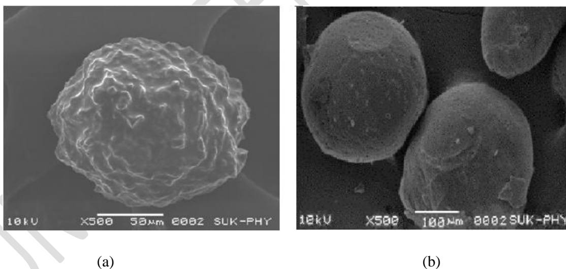
Fig 1. SEM micrograph of microparticle prepared 1:5 drug: TKP ratio (a) uncoated microspheres (T5) (b) Eudragit S-100 coated microspheres (ET5)
