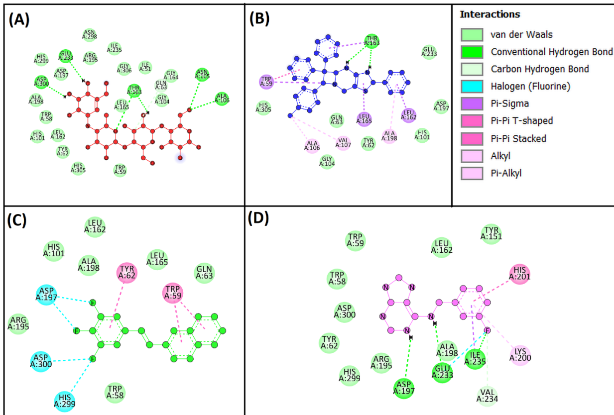
Figure 2. Molecular interactions analysis of best docked ligands with \alpha -amylase (2QV4) enzyme. (A) Redocked acarbose; (B) C7 compound; (C) C4 compound; (D) C3 compound.
