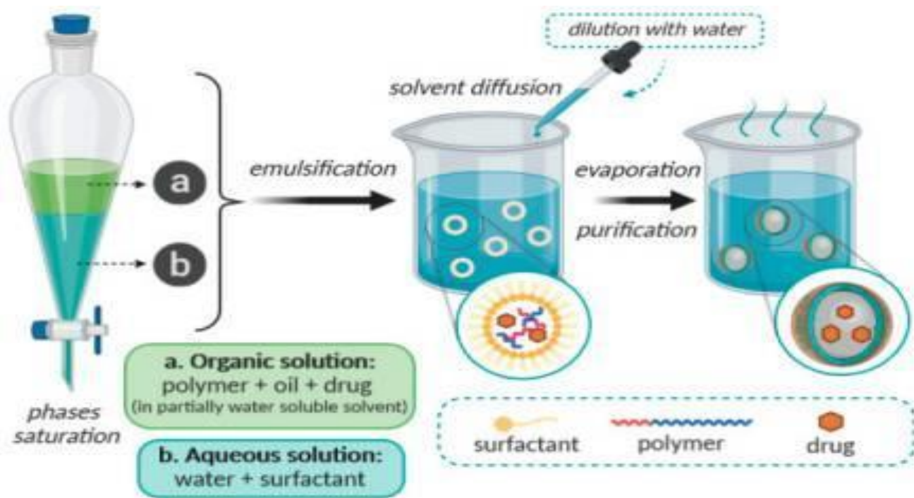
Fig No.3 Graphical representation of solvent diffusion method
