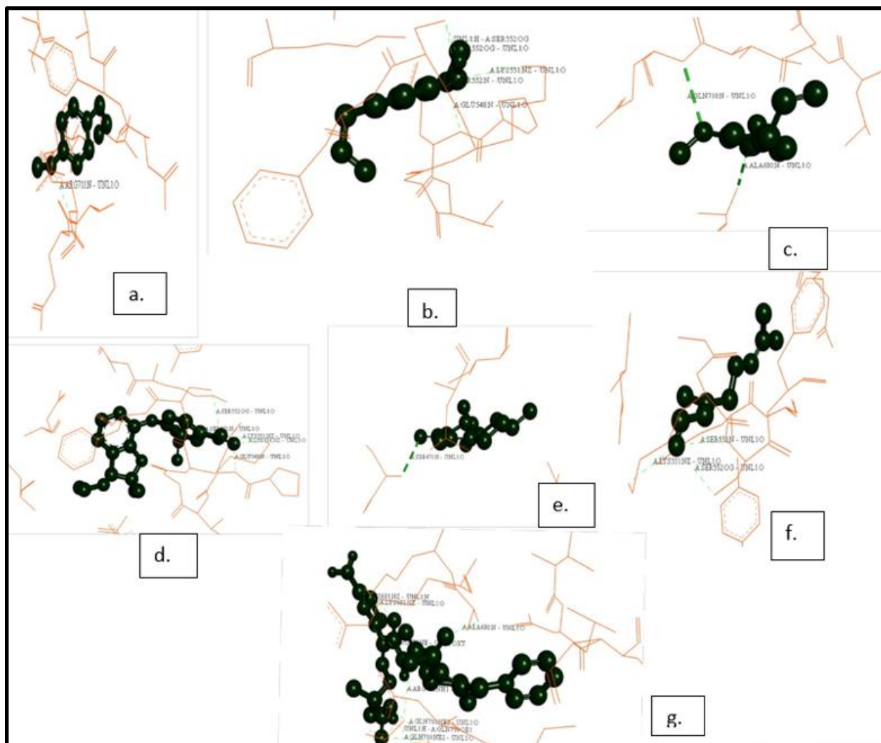
Figure-3- 3D diagrams showing the bond interactions between the essential compounds from Ocimum sanctum and PTK of A. baumannii a.Estragole b.Eugenol c.Methyleugenol d.Benzofuran, 7-(2,4- dinitrophenoxy)-3-ethoxy-2,3- dihydro-2,2-dimethyl e.Hexahydro-1,6-dimethyl-4- (1-methylethyl)- f.Citral g.Ceftazidime
