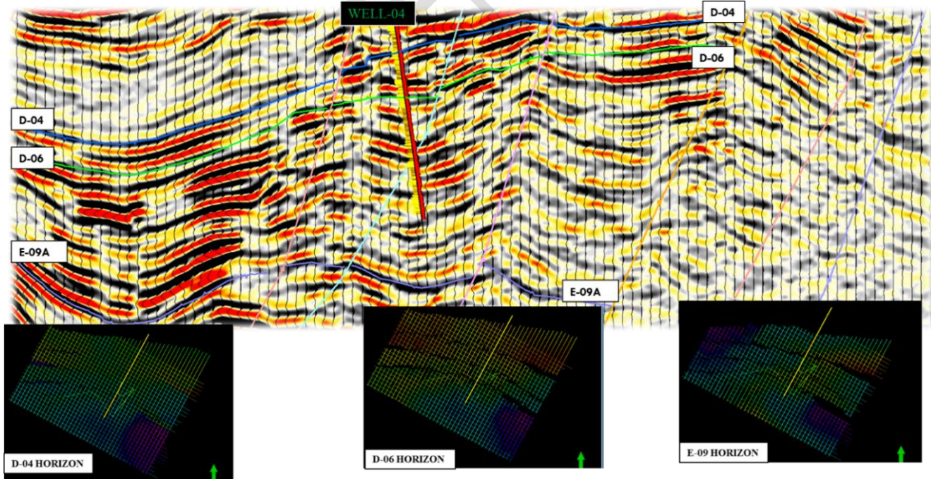
Fig. 6b. 2-D window showing the different horizons mapped across the field
