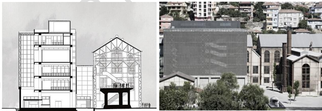
Figure 12. Santral Istanbul sectional and facade view [URL-4]
