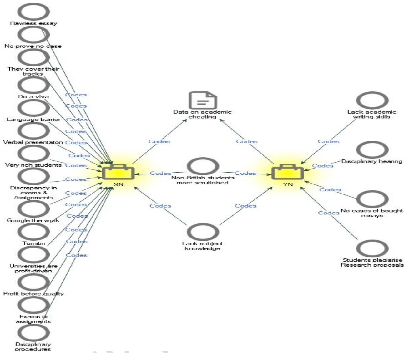
Figure 2. Comparison between SN and YN
