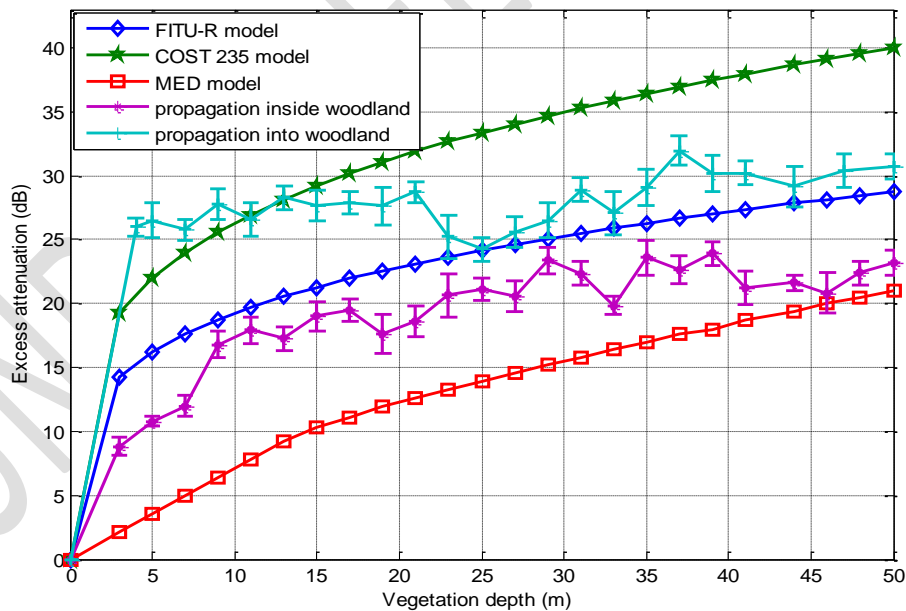
Figure 2.0 Excess loss versus depth for propagation (into and inside) woodland at 5.0 GHz
