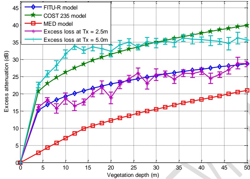
Figure 4.0 Excess loss at two antenna heights compared with empirical models at 5.0 GHz.
