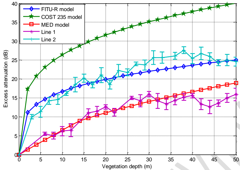
Figure 6.0 Excess attenuation for lines of trees at 3.5 GHz
