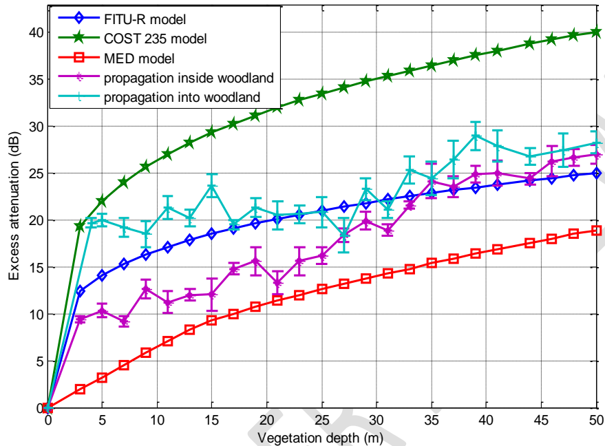
Figure 1.0 Excess loss versus depth for propagation (into and inside) woodland at 3.5 GHz
