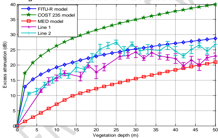
Figure 7.0 Excess attenuation for lines of trees at 5.0 GHz
