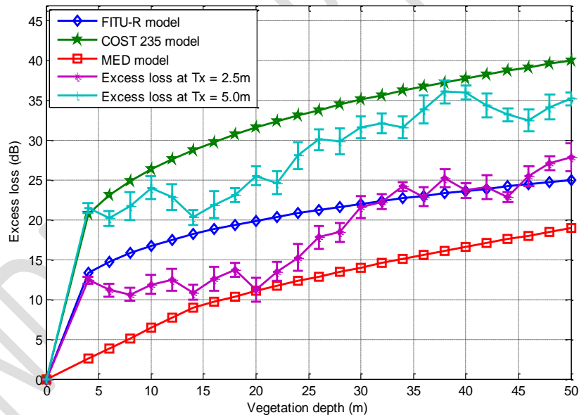
Figure 3.0 Excess loss at two antenna heights compared with empirical models at 3.5 GHz
