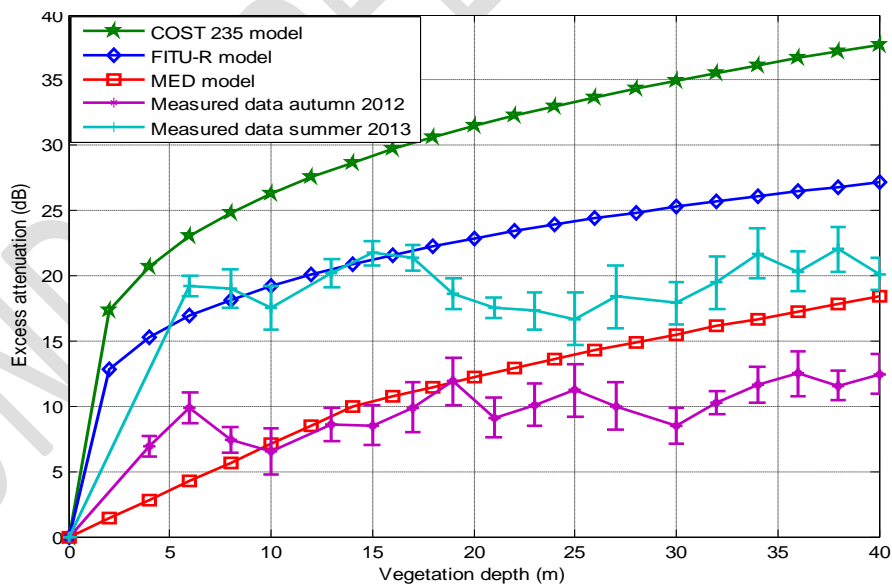
Figure 3.0 Excess attenuation versus depth in autumn and summer at 5.0 GHz for path 1
