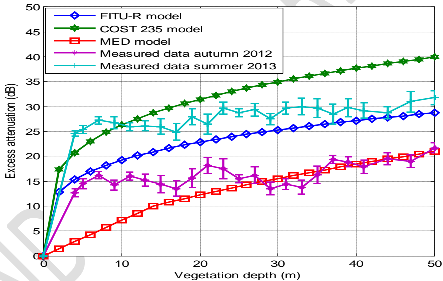
Figure 5.0 Excess attenuation versus depth at 5.0 GHz for path 2
