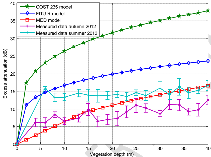
Figure 2.0 Excess attenuation versus depth in autumn and summer at 3.5 GHz for path 1
