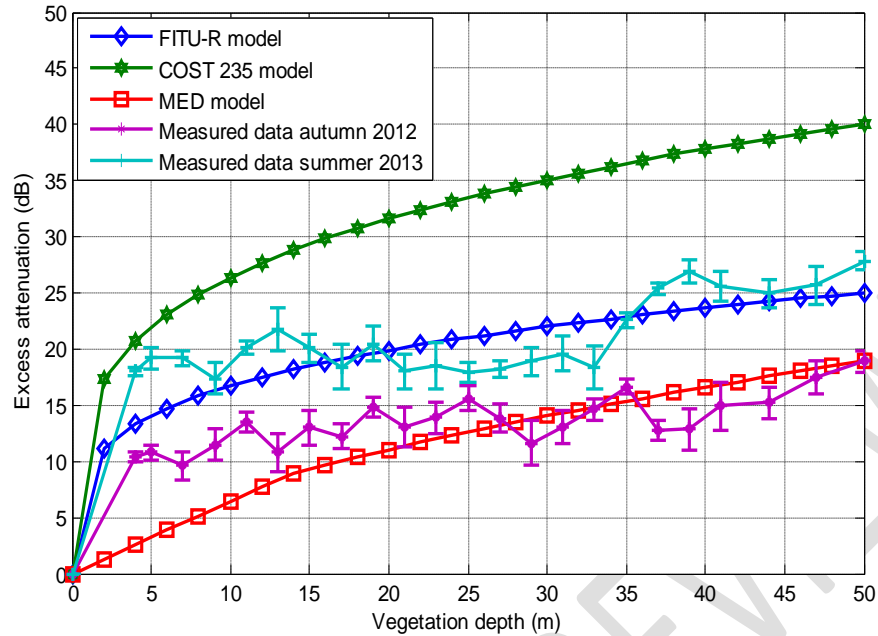
Figure 4.0 Excess attenuation versus depth at 3.5 GHz for path 2
