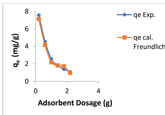
Figure 2: Freundlich plot of q_{e-Exp.} Vs q_{e-Cal}
