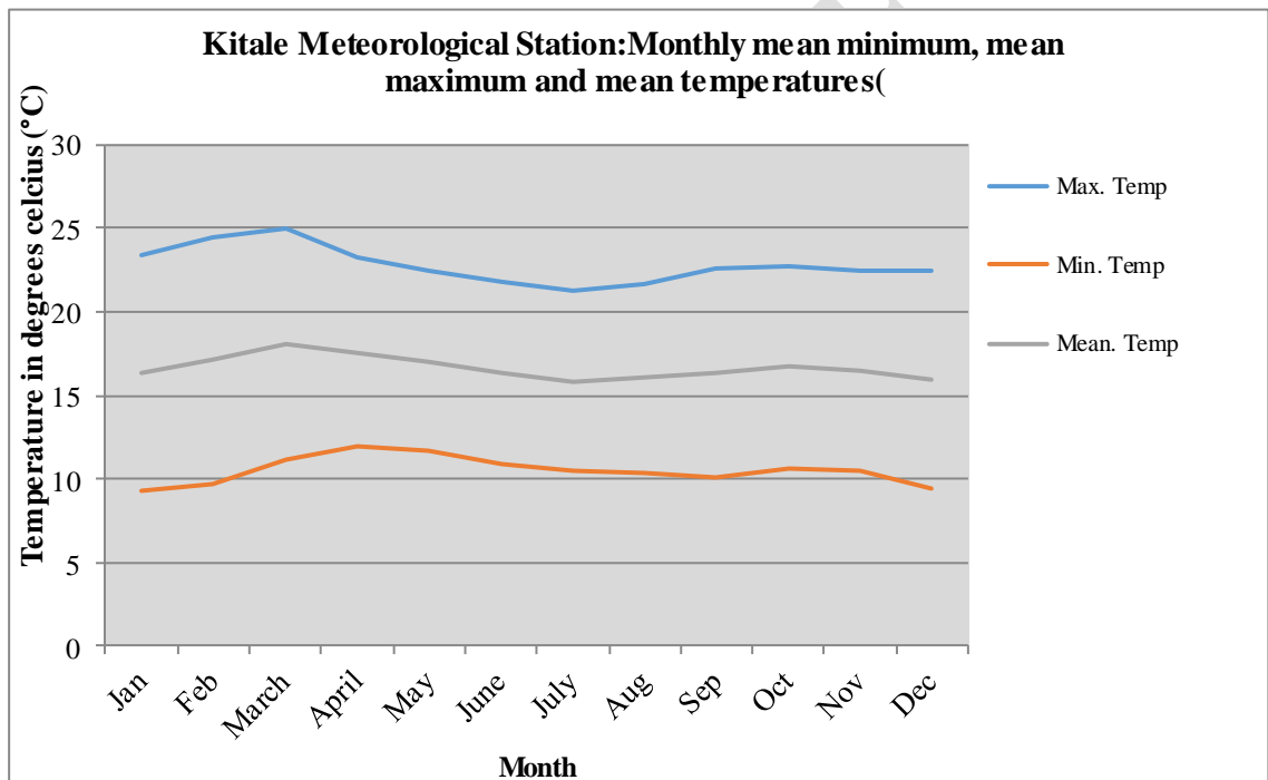
Figure 4: Comparison of monthly mean minimum, mean maximum and mean temperatures for Kitale meteorological station between 1979 and 2014
