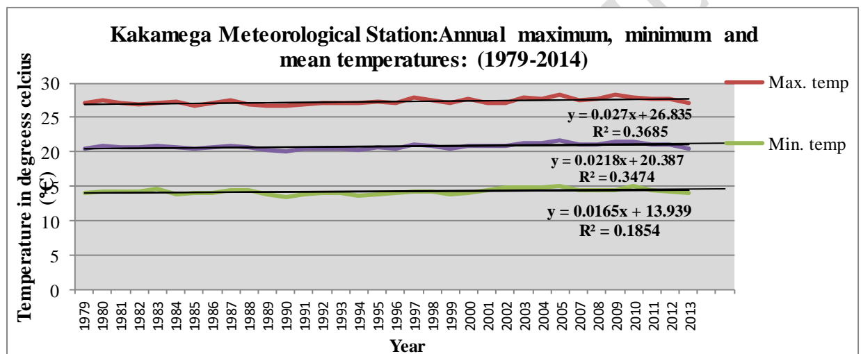
Figure. 12: Comparison of annual minimum, maximum and mean temperatures trends for Kakamega meteorological station
