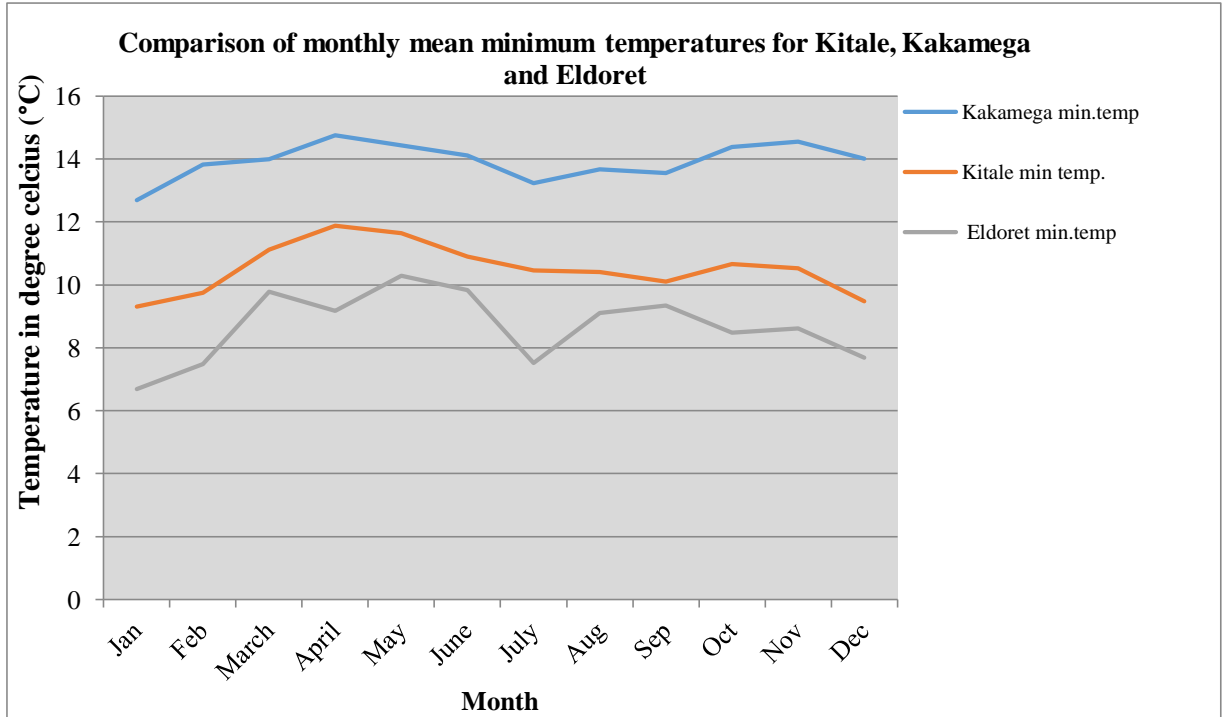
Figure 7: Comparison of monthly minimum temperatures for Kitale, Kakamega and Eldoret international airport meteorological stations
