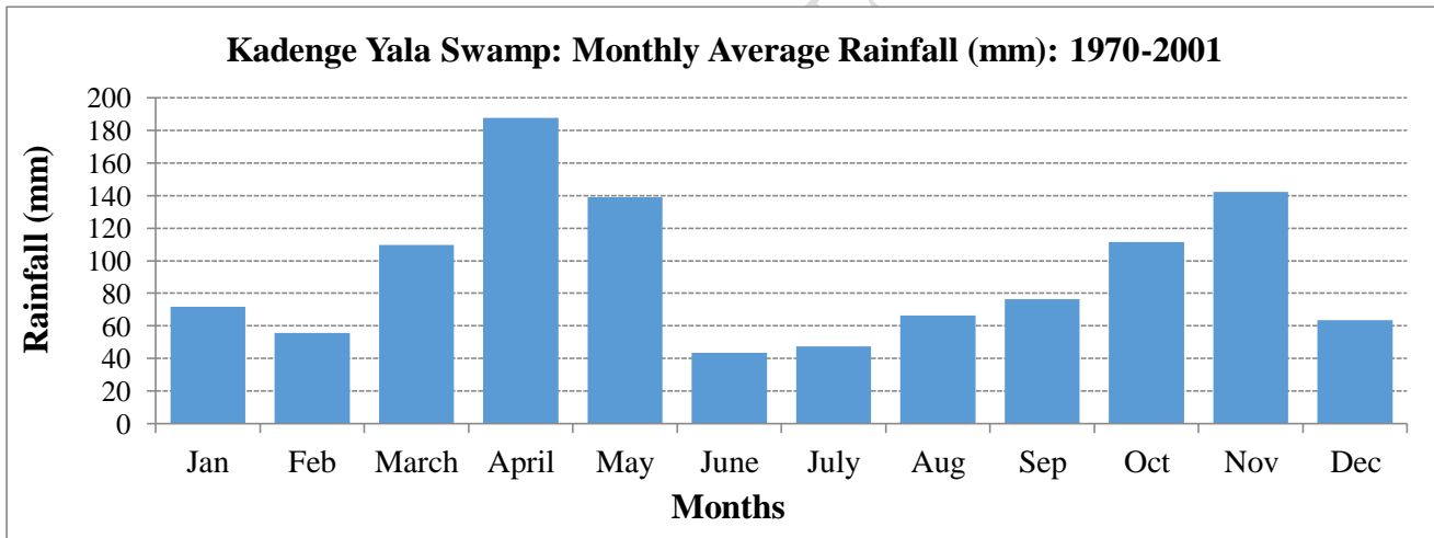
Figure. 2: Monthly average rainfall distribution for selected rainfall stations within Nzoia River Basin, Kenya.
