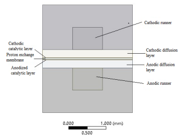
Fig. 2. Schematic diagram of the fuel cell structure
