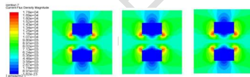
Fig. 13. Current density distribution at the intermediate section
