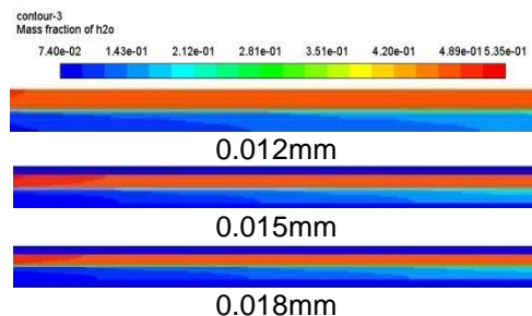
Fig. 11. Lateral water mass distribution
