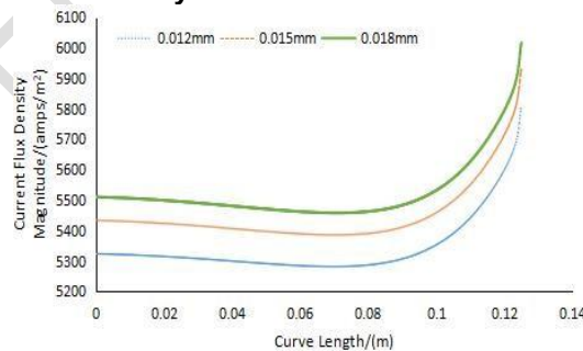
Fig. 13. Current density distribution at the intermediate section
