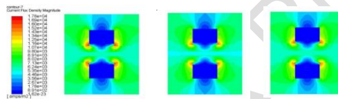
Fig. 7. Distribution of current density in the middle of different GDL thicknesses
