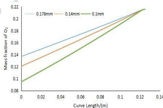
Fig. 16. Mass distribution curve of oxygen in the cathode runner
