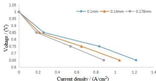
Fig. 17. Polarization curves of different proton exchange membranes
