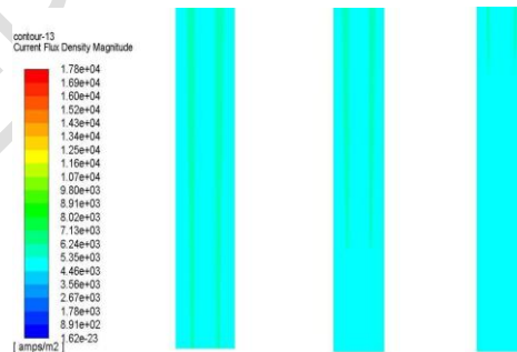
Fig. 8. Distribution of current density on the proton exchange membrane near the inlet position
