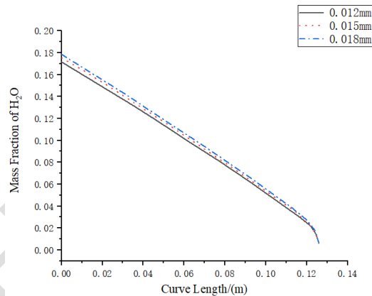
Fig. 10. Distribution of water content in the cathode diffusion layer
