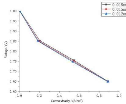
Fig. 12. Polarization curves of fuel cells with different catalytic layer thicknesses
