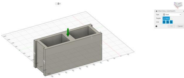
Figure 5. A The uniform application of pressure on the topside of the Hollow Block
