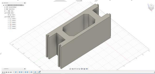
Figure 3.D The Third Proposed Design (Design C)
