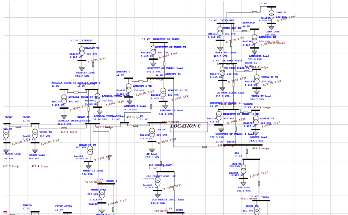
Figure 4: Location C on ETAP reliability run mode
