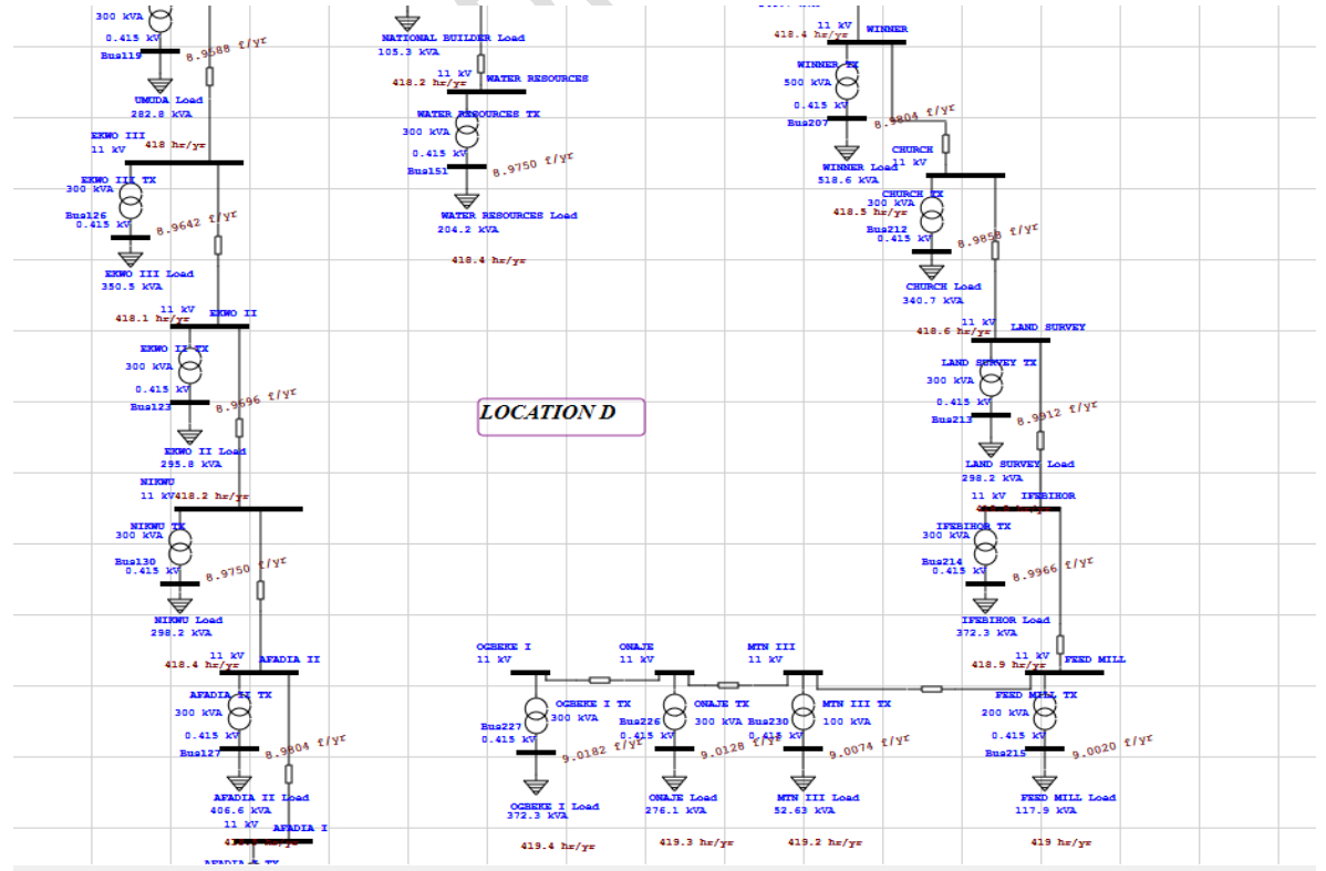
Figure 5: Location D on ETAP reliability run mode
