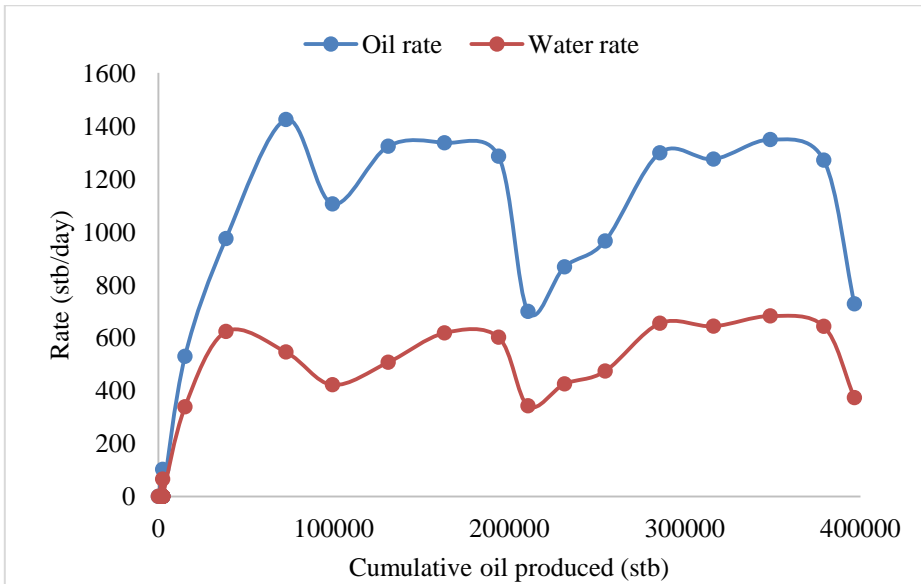
Fig. 5. Oil and water Rates Production against Cumulative Oil Production. (Well 3L)
