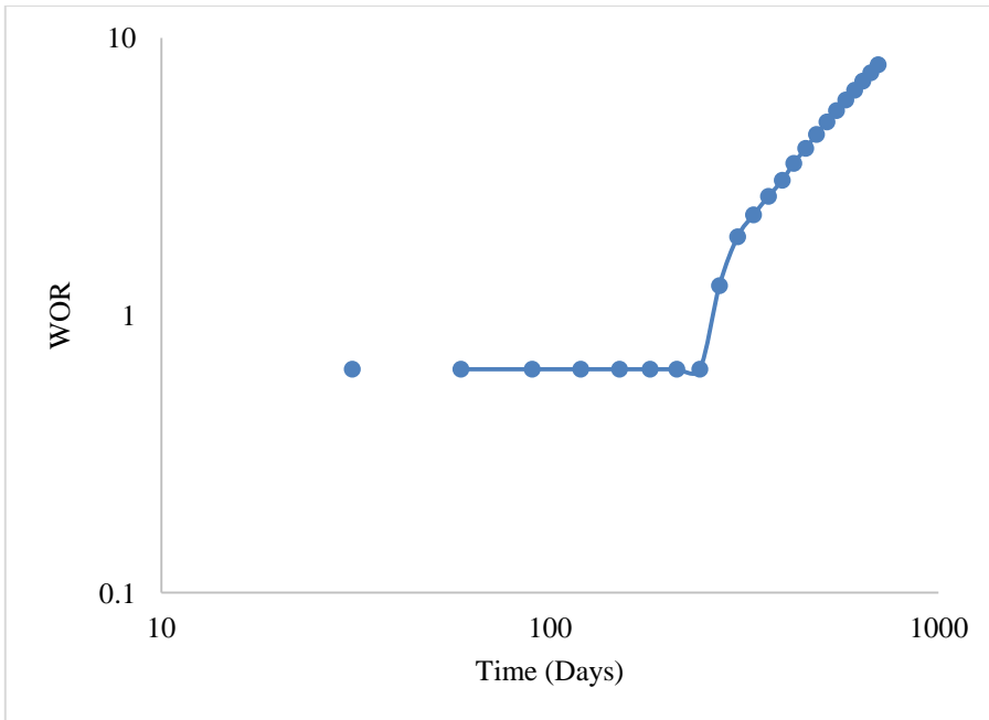
Fig. 7. Log-Log Plot of WOR against Time Showing Multilayer Channeling (Well 3L).
