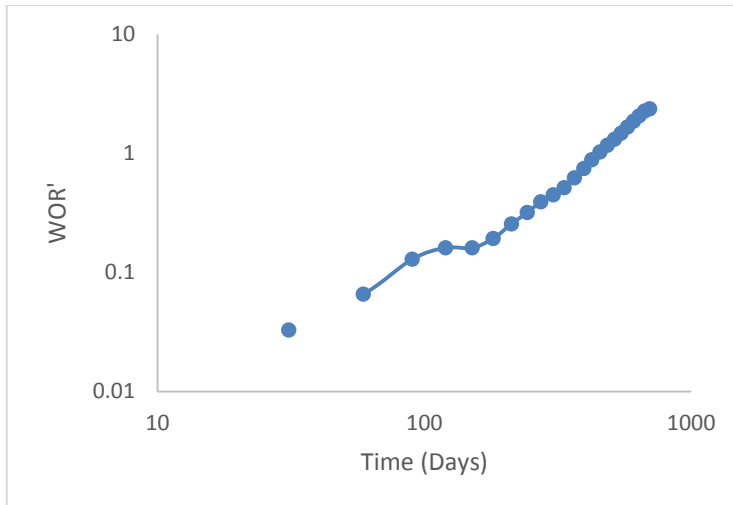
Fig. 3. Log-Log Plot of WOR Derivative against Time Showing Channeling Behind Casing. (Well 3S)
