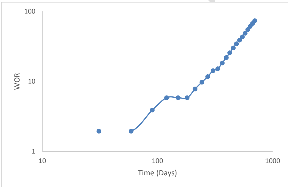
Fig.2. Log-Log Plot of WOR against Time Showing Channelling Behind Casing. (Well 3S)
