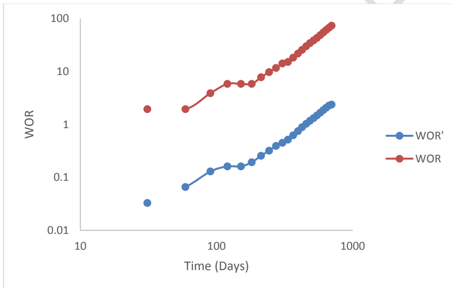
Fig. 4. Log-Log Plot of WOR and WOR Derivative against Time. (Well 3S)
