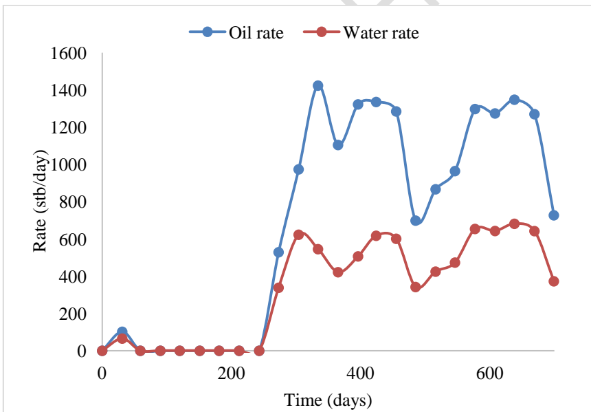
Fig. 6. Oil and water Rates Production against Time. (Well 3L)
