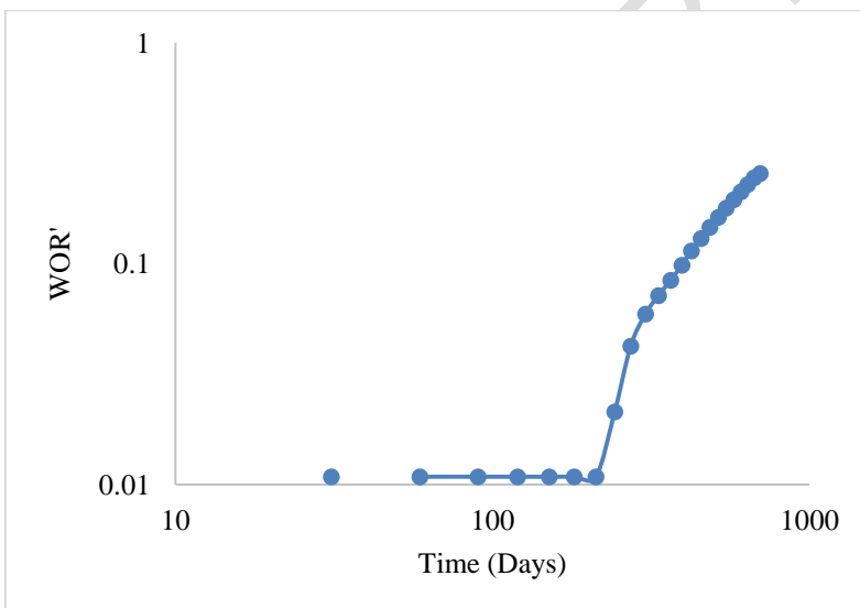
Fig.8. Log-Log Plot of WOR Derivative against Time Showing Multilayer Channeling (Well 3L).
