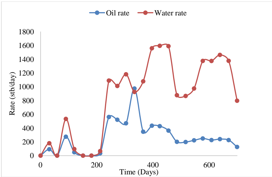
Fig. 1. Oil and water Rates Production against Time. (Well 3S)
