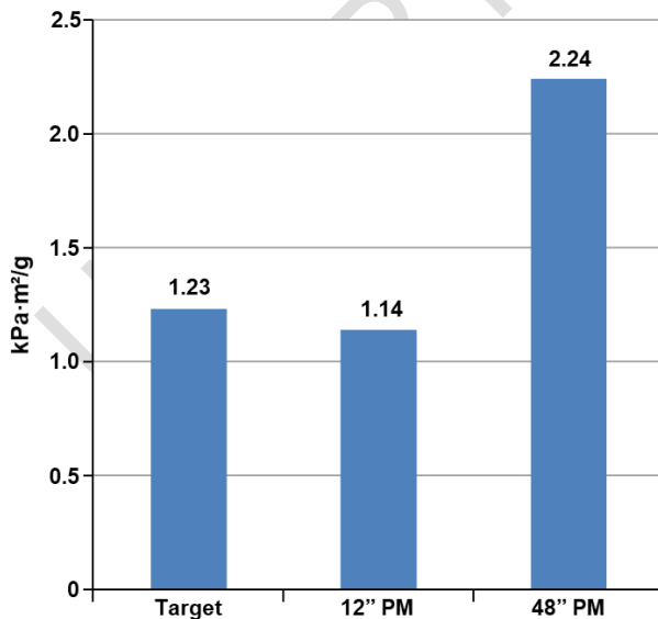
Fig. 11. Paper machine run burst index
