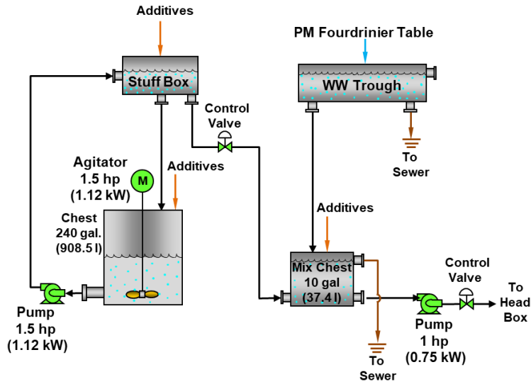
Fig. 5. Wet End of the 12" laboratory Fourdrinier paper machine [31].
