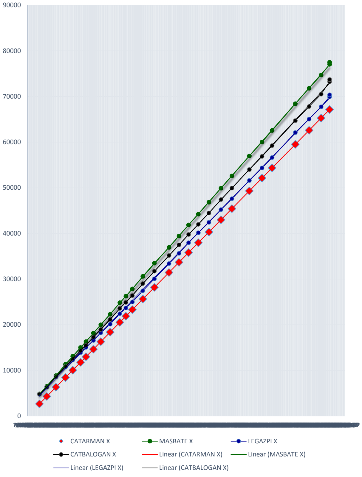
FIGURE 1. DOUBLE MASS ANALYSIS CURVE
