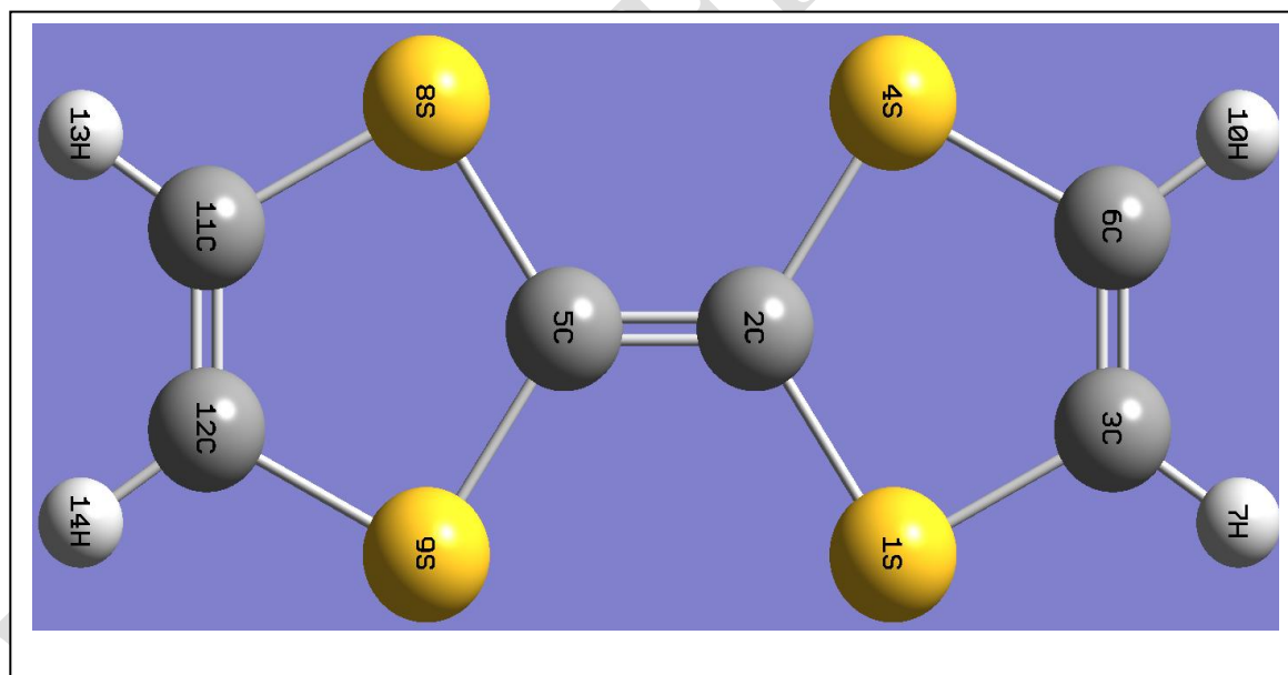
Figure 1: optimized structure of TTF molecule.
