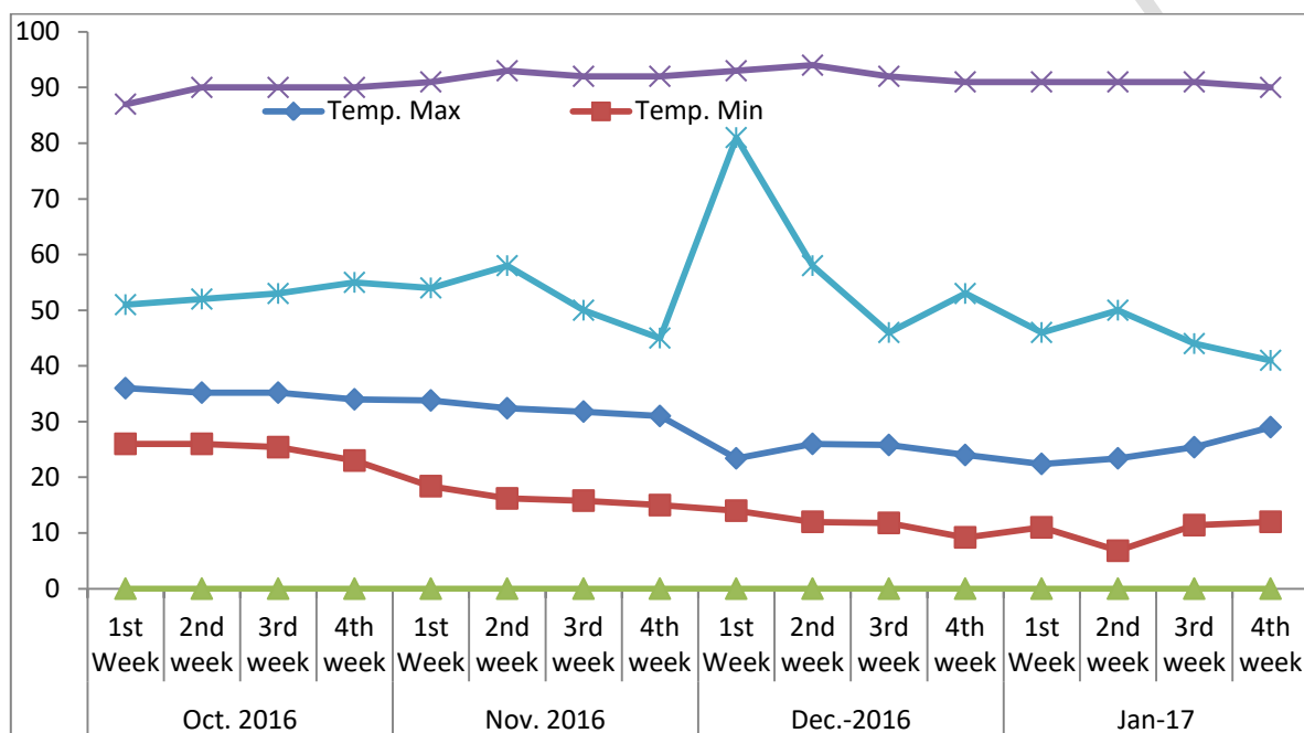
Fig.-1 Meteorological data (October 2016 – January 2017).
