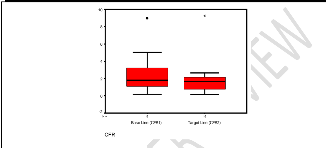
Fig 1: Box-Whisker plot
