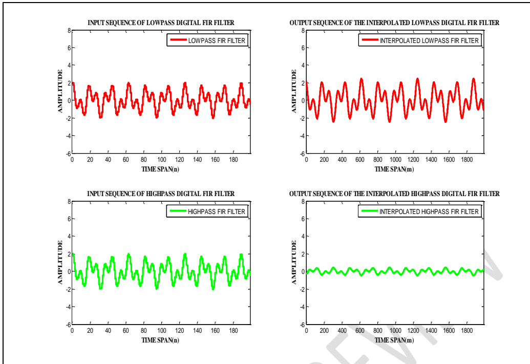
Figure 10: MATLAB Implementation of the Interpolation Process
