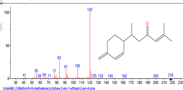
Fig. 2f. Mass spectrum of 2-Methyl-6-(4-methylenecyclohex-2-en-1-yl)hept-2-en-4-one structure.
