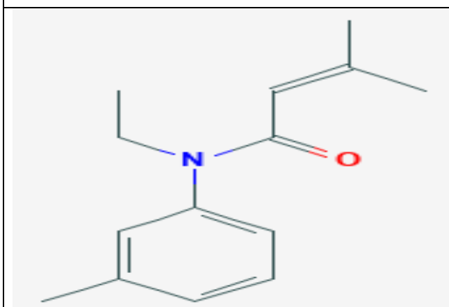
Fig. 2q. Structure of But-2-enamide, N-ethyl-N-(3-methyl phenyl)-3-methyl-
