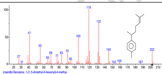
Fig. 2d. Mass spectrum of Benzene, 1-(1,5-dimethylhexenyl)-4-methyl- structure.
