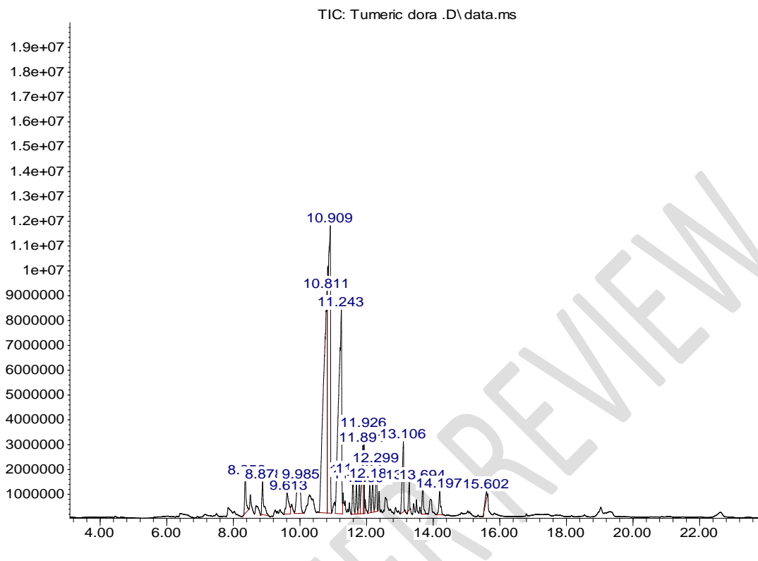
Figure 1: Gas-Chromatography–Mass Spectrometry chromatogram of Turmeric ( Curcuma longa )
