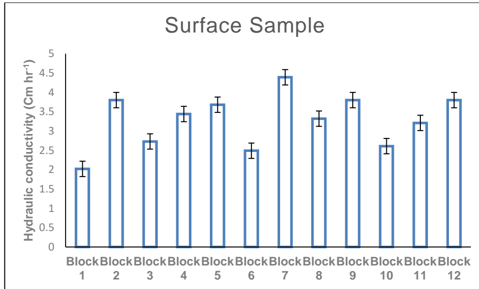
Fig 2. Effect of paper board industry effluent irrigated soils on Hydraulic conductivity (Ks) (cm hr -1 ) of surface soil
