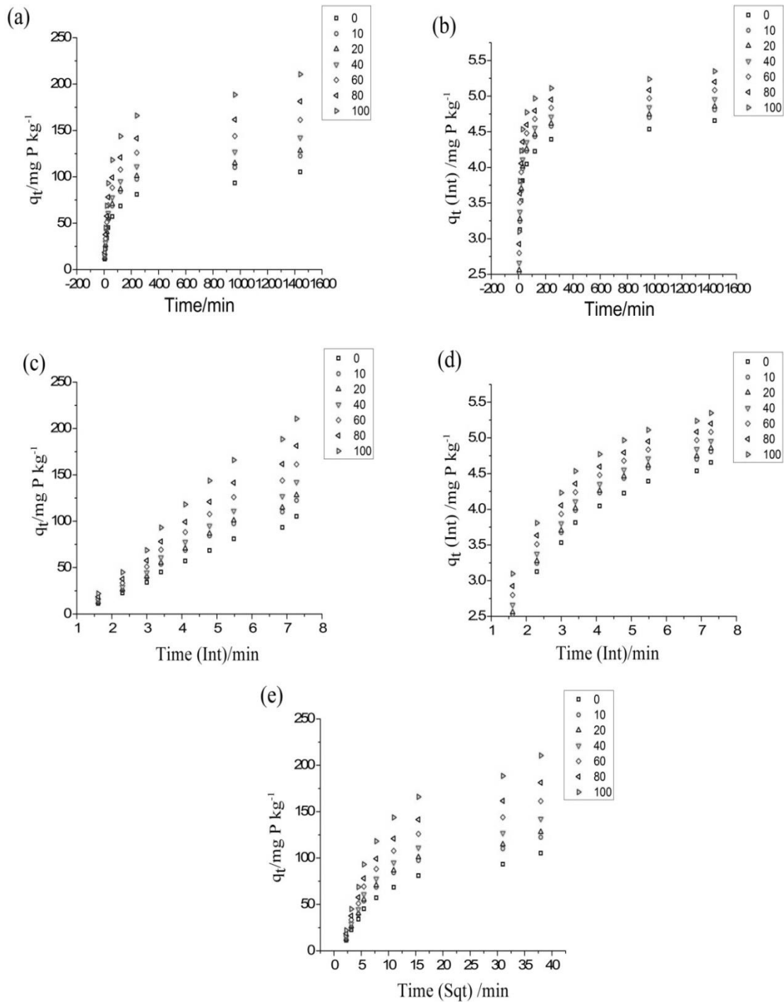
Fig 2. The kinetics of P release by citric acid applied at 0, 10, 20, 40, 60, 80, 100 mM concentrations in highly calcareous soil having 21.5% free CaCO 3 as a function of time and similar data described by five kinetic models: Zero-order (a), First order (b), Simple elovich (c), Power (d) and parabolic functions (e)
