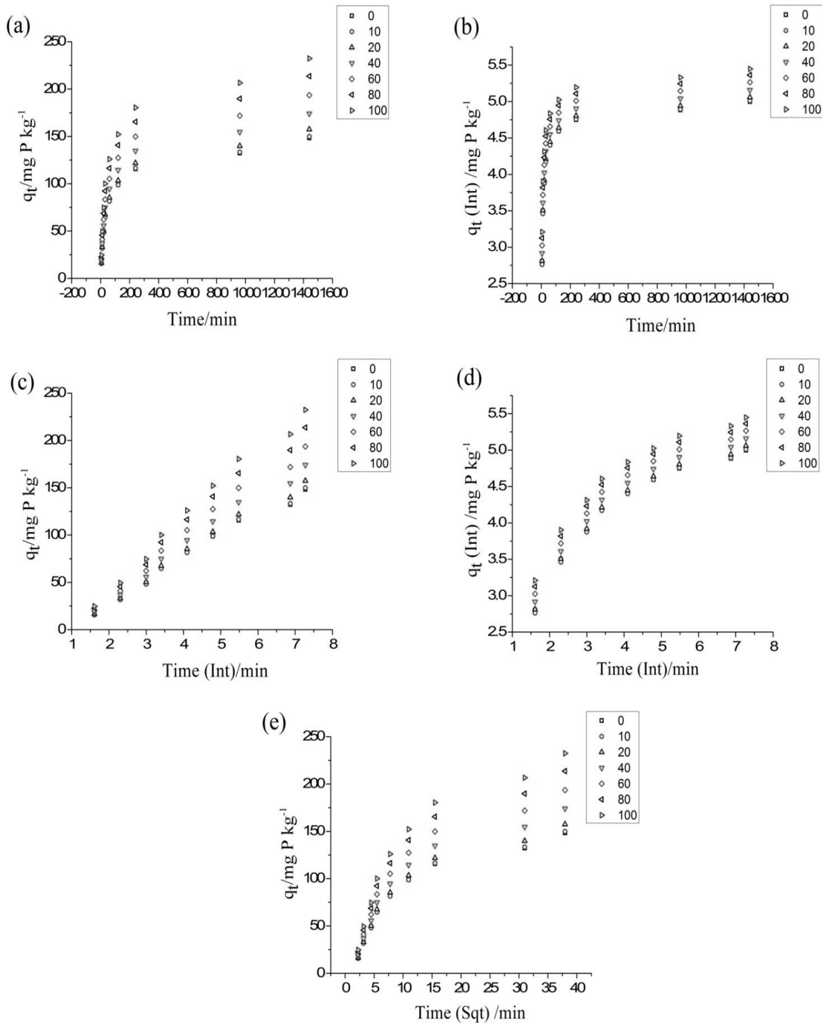
Fig1. The kinetics of P release by citric acid applied at 0, 10, 20, 40, 60, 80, 100 mM concentrations in highly calcareous soil having 17.5% free \text{CaCO}_3 as a function of time and similar data described by five kinetic models: Zero-order (a), First order (b), Simple elovich (c), Power (d) and parabolic functions (e)
