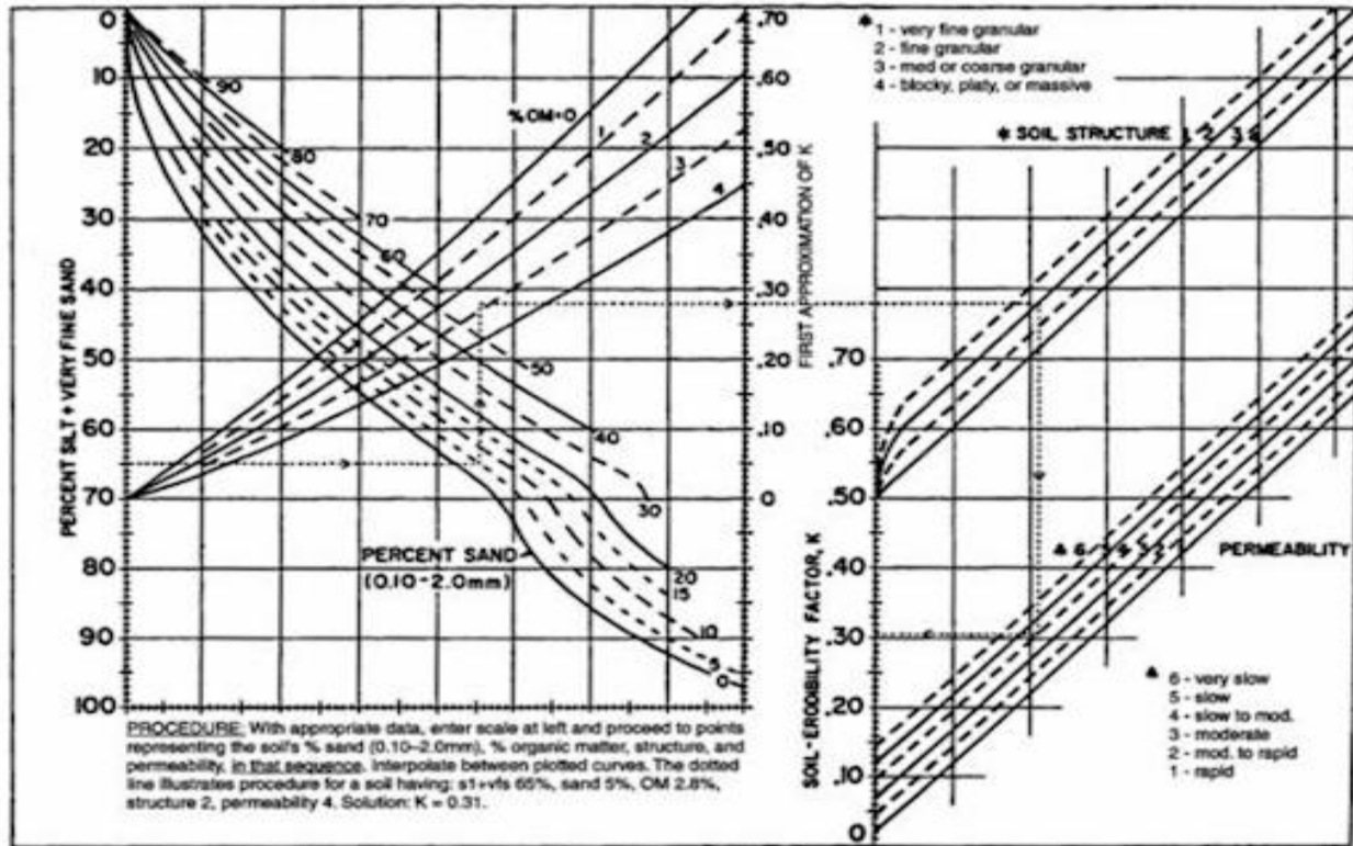
Figure 1. Soil nomogram - erodability. Foster et al, 1981.
