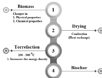
Fig. 4 Steps involved in biochar production process by thermochemical methods [30].
