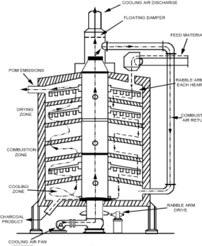
Fig.6 Continuous multiple hearth kiln[36]
