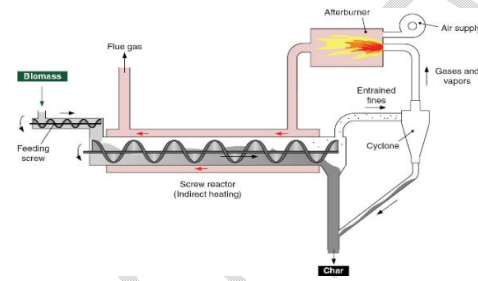
Fig. 3 Continuous Type Biochar reactor[31]
