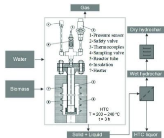
Fig.1 Hydrothermal Carbonization reactor
