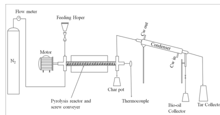
Fig. 7 Continuous screw auger Biochar reactor [37]
