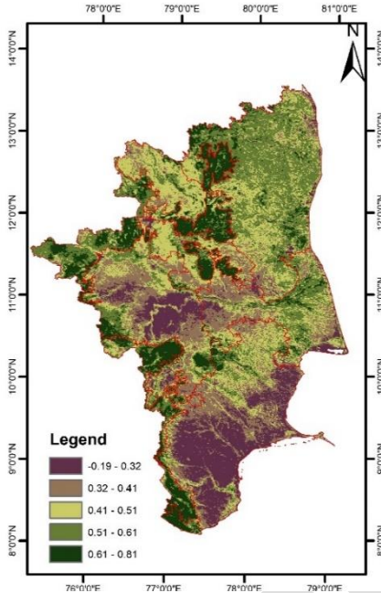
Fig. 7: Spatial Distribution of NDVI during SWM (2011-20)
