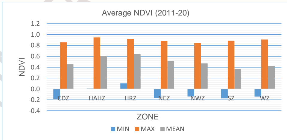
Fig. 4: Average NDVI (2011-20) during SWM
