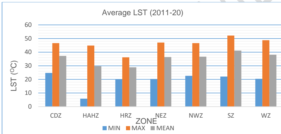
Fig. 3: Average LST (2011-20) during SWM
