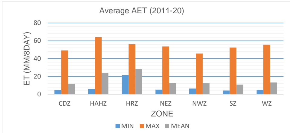
Fig. 2: Average AET (2011-20) during SWM
