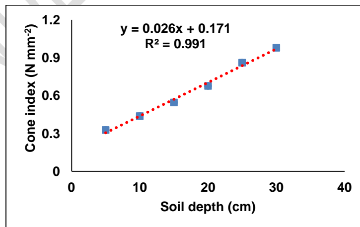
Fig. 2. Relationship between cone index and soil depth
