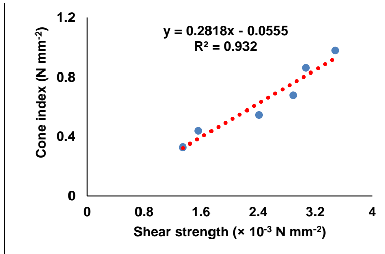
Fig. 4. Relationship between shear strength and cone index
