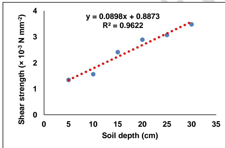
Fig. 3. Relationship between shear strength and soil depth
