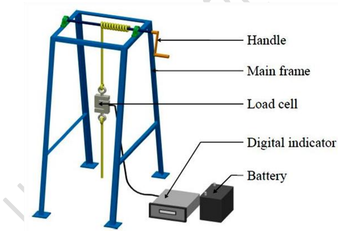
Fig. 1. Pulling force measuring apparatus
